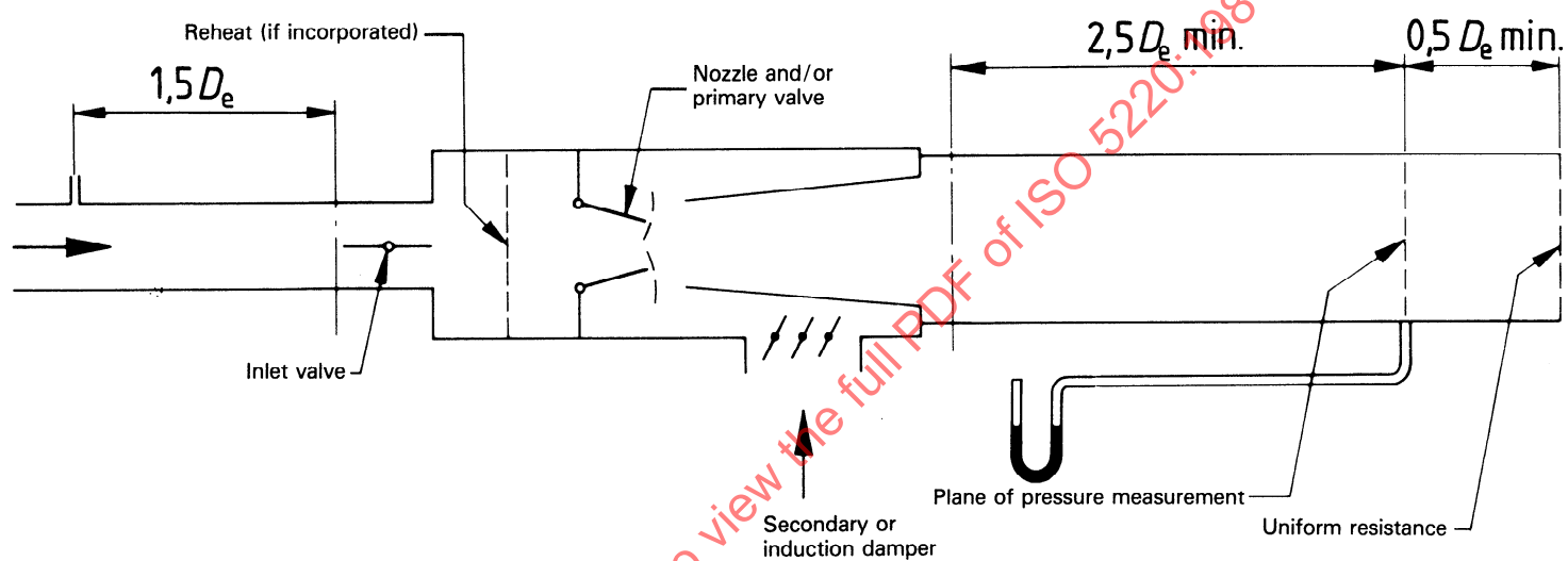
Figure 7 — Typical induction box test installation
