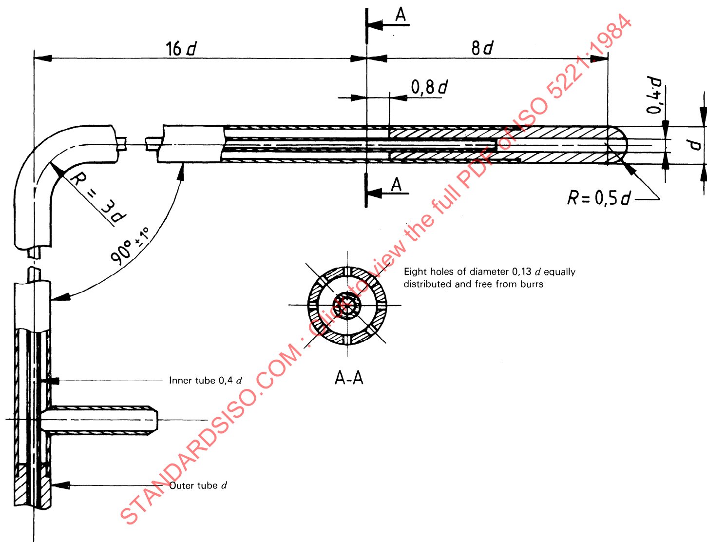
Figure 19 — Pitot-static tube, type AMCA
