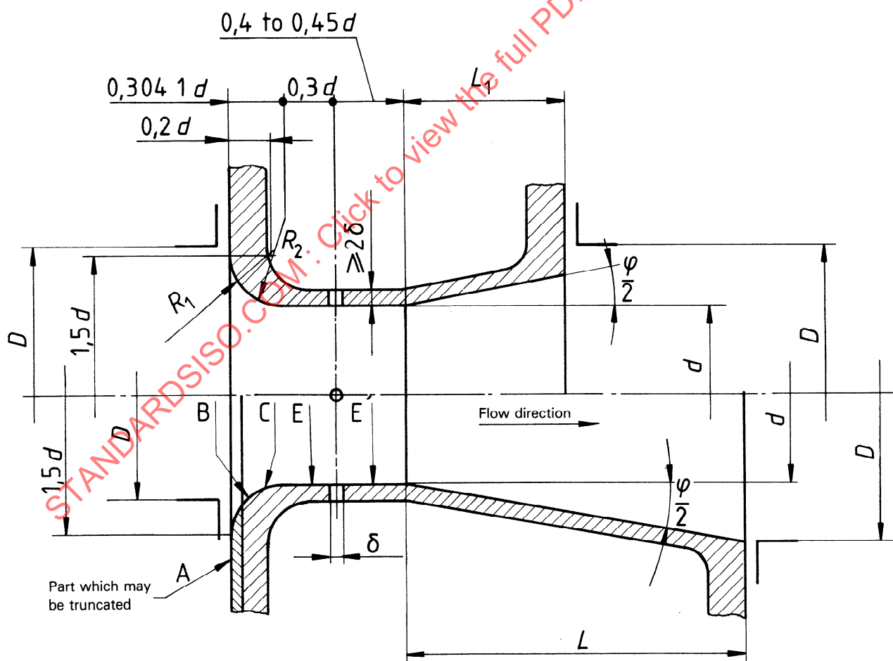
Figure 9 — Venturi nozzle
