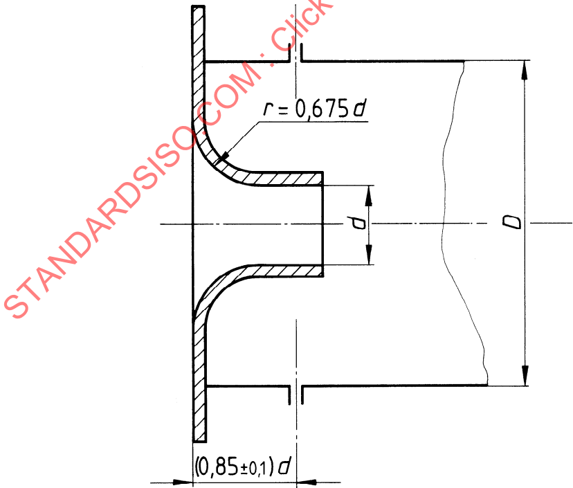
Figure 15 — “Quarter-circle” nozzle located at the inlet end of the system
