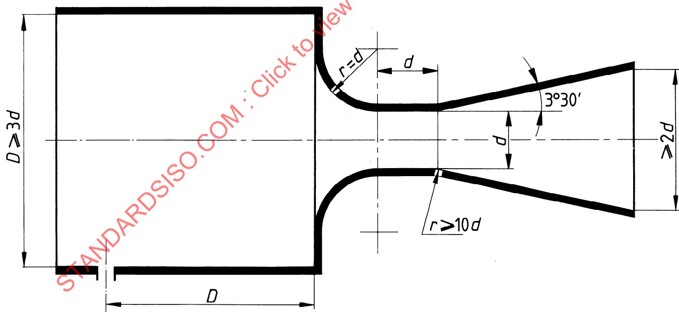
Figure 18 — Venturi-nozzle with sonic throat type "LMEF"
