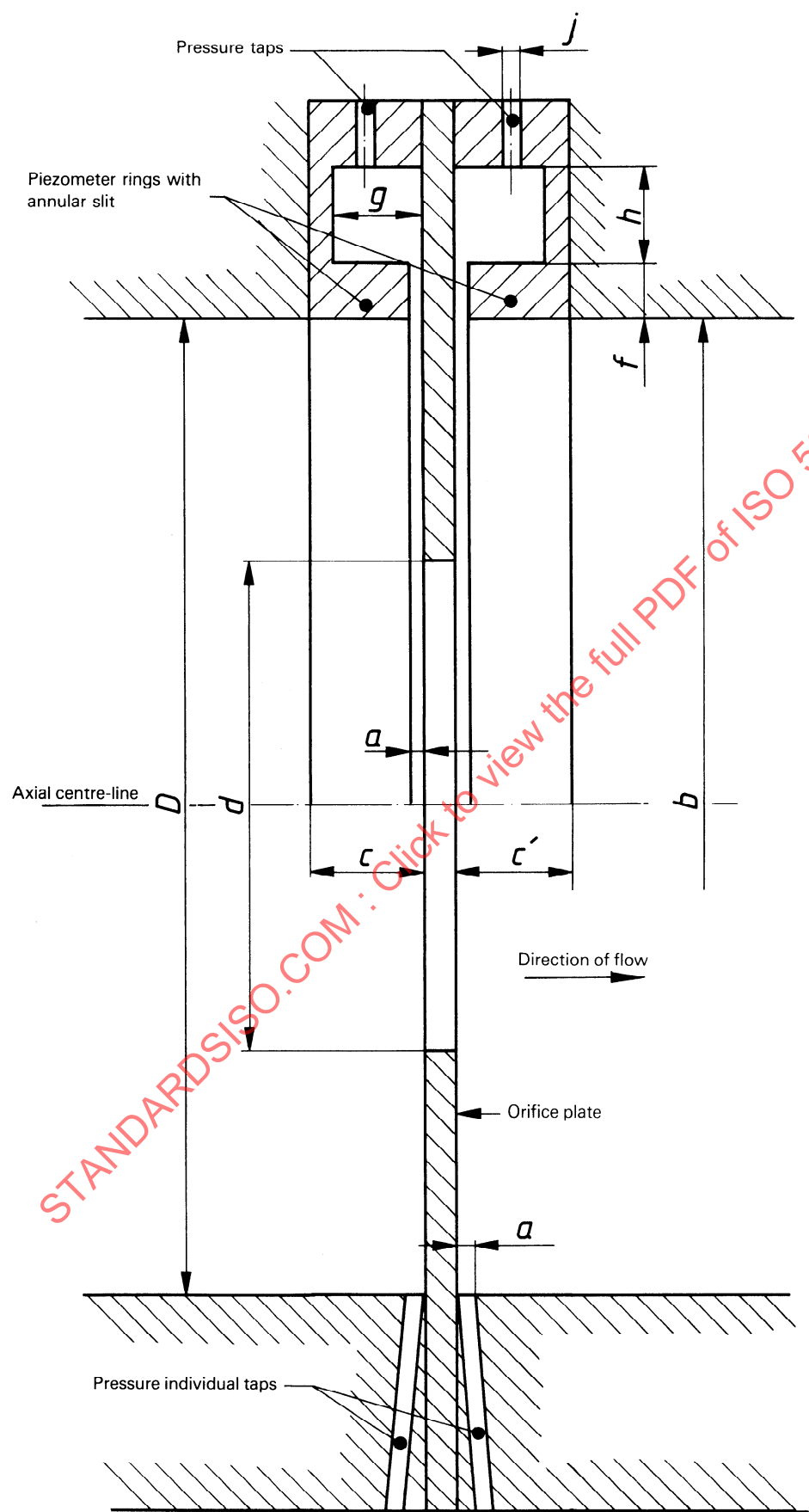
Figure 3 – Corner taps
