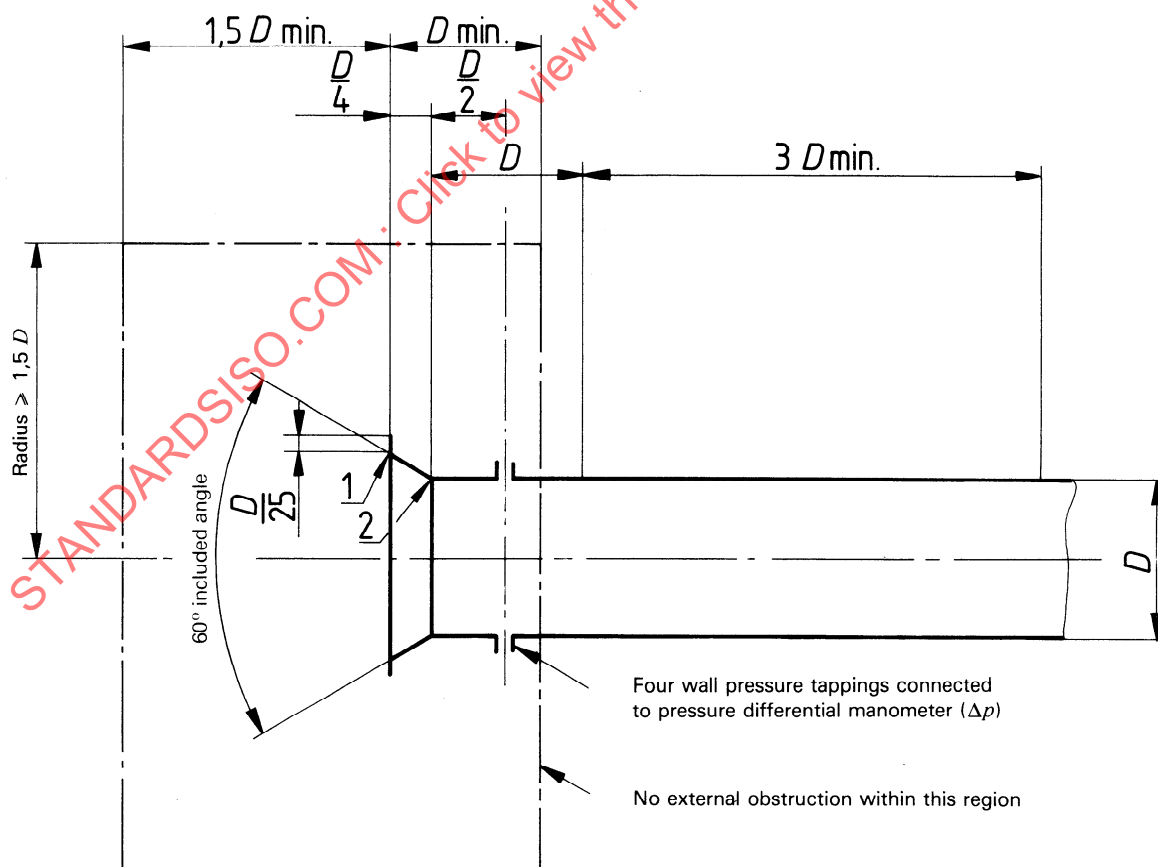
Figure 16 — Inlet cone
