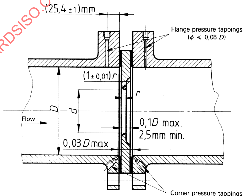
Figure 11 — "Quarter-circle" orifice plate
