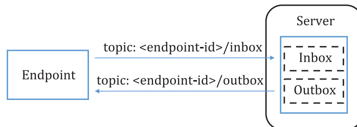
Figure 19 — Communication with Server using MQTT
