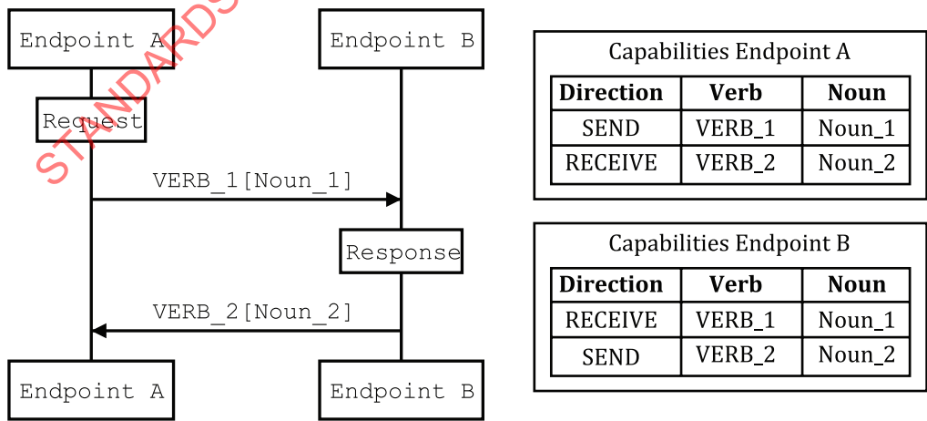
Figure 11 — Necessary capabilities to support a scenario
