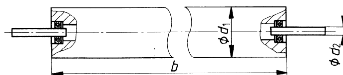
Figure 2 — Type B: Fixed spindle
