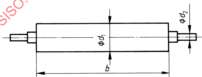
Figure 1 — Type A: Revolving spindle
