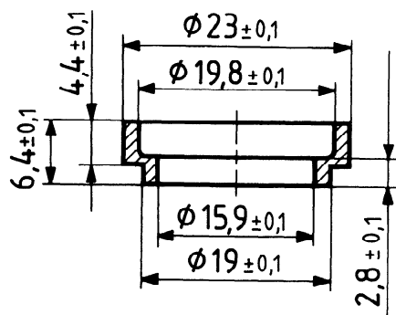
Figure 1 — Ring (see D.2.1)
