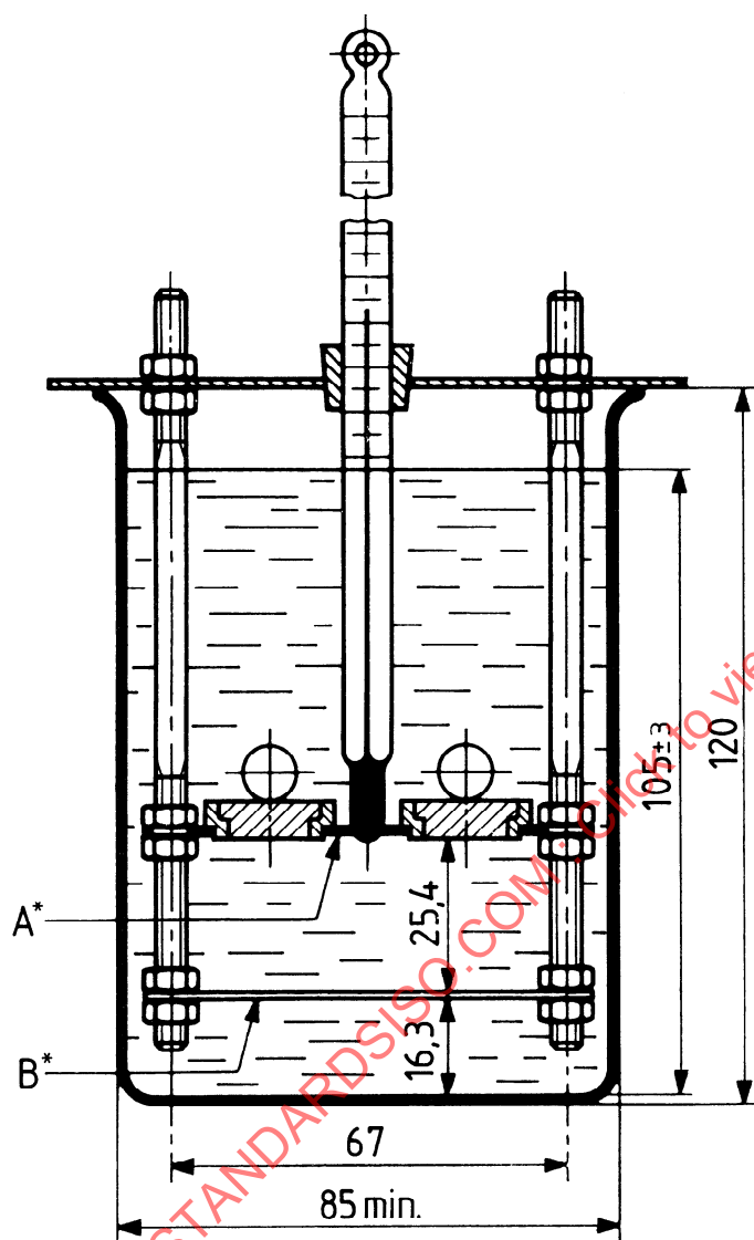
Figure 3 — Ring and ball apparatus (see D.2.6)
