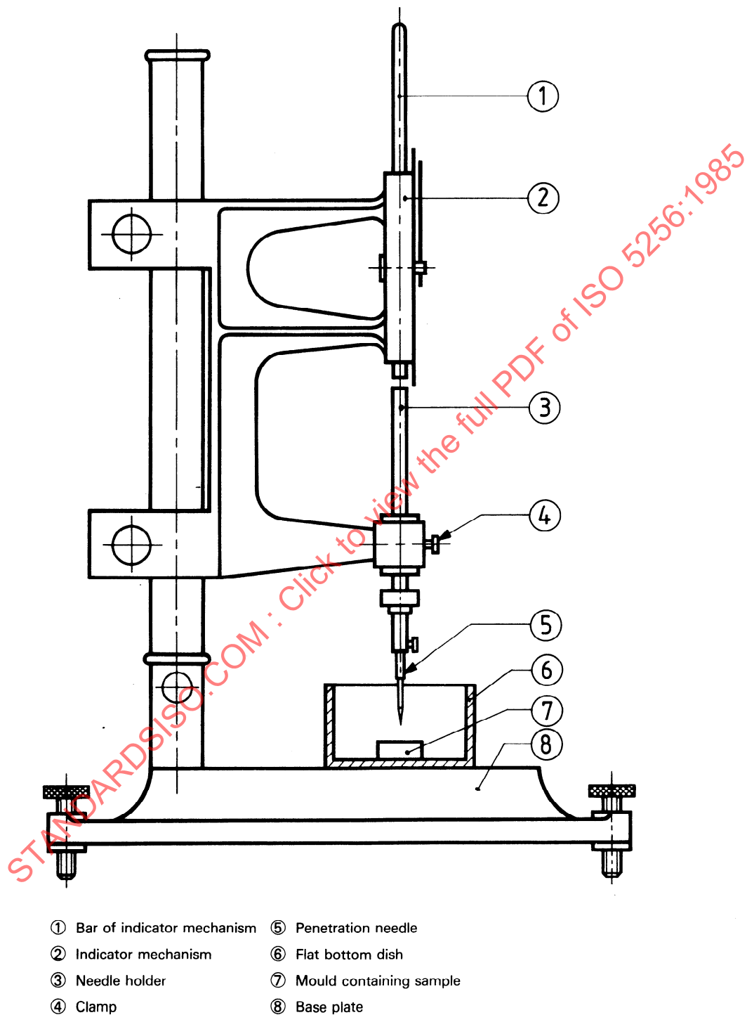
Figure 5 — Penetrometer (see E.2.1)
