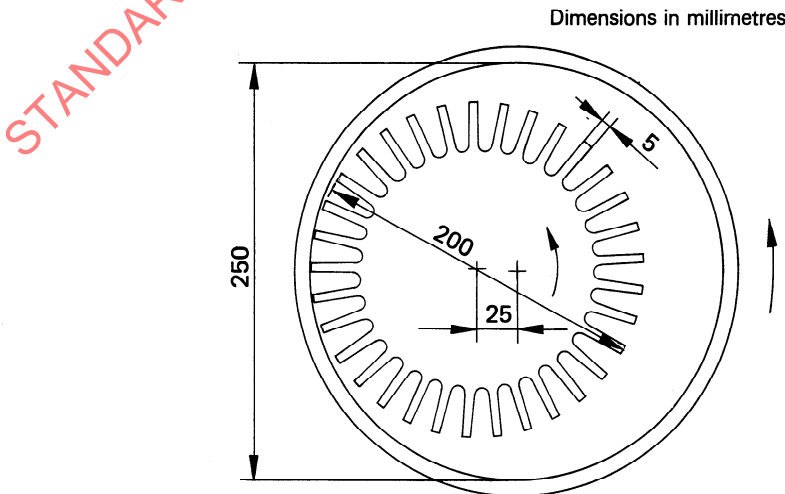
Figure — Principal elements of the PFI mill
