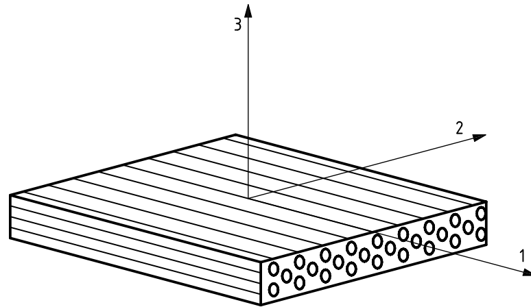
Figure 2 — Fibre-reinforced plastic composite showing axes of symmetry
