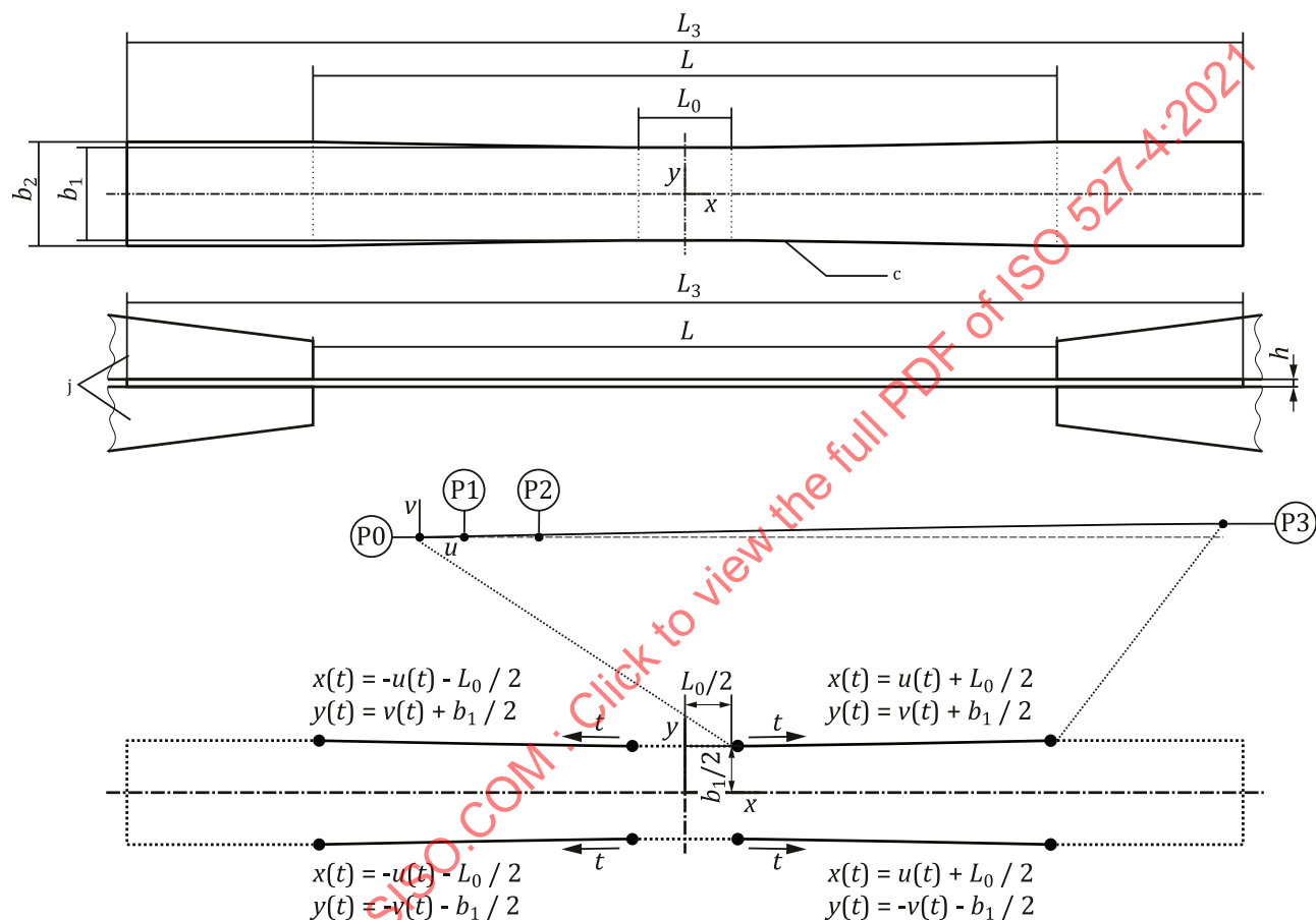
Figure 4 — Type 2 and type 3 specimens
