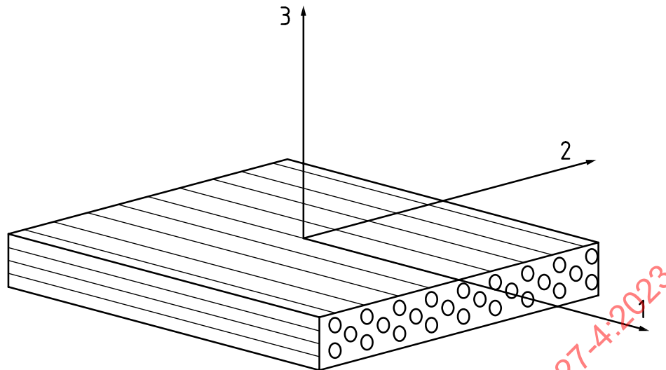
Figure 2 — Fibre-reinforced plastic composite showing axes of symmetry
