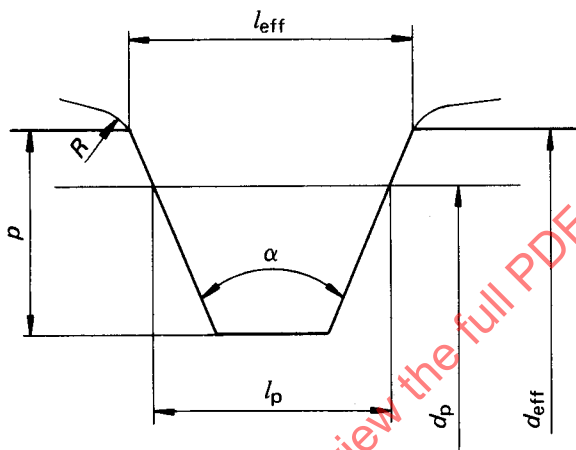
FIGURE 1 — Test pulley
