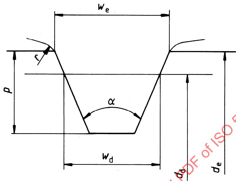
Figure 1 — Test pulley groove
