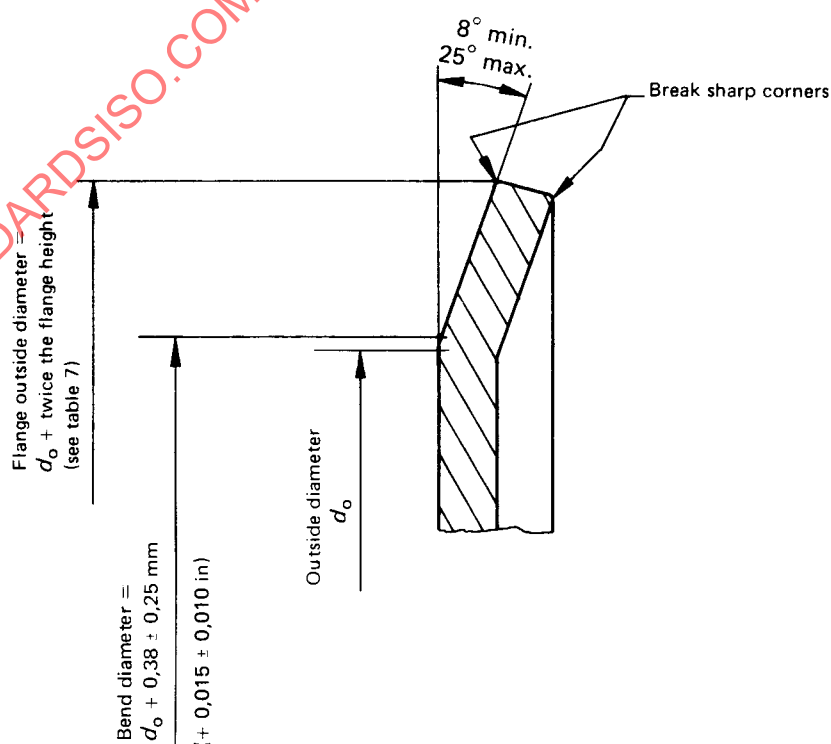
Figure 4 — Flange dimensions
