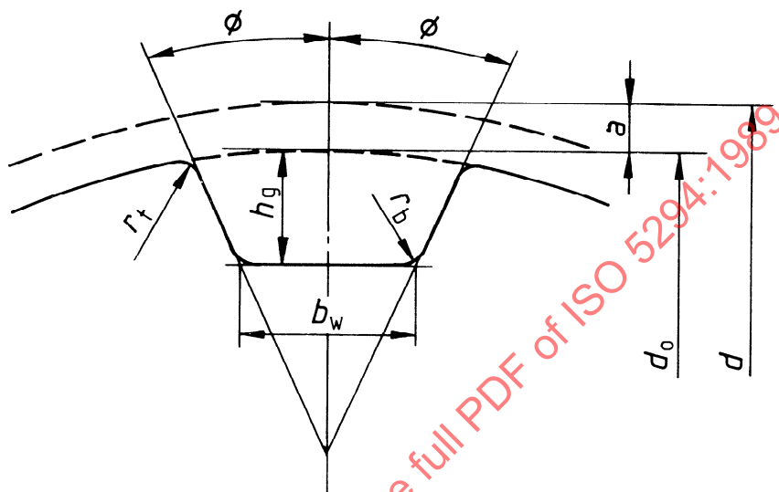
Figure 2 — Straight-sided teeth
