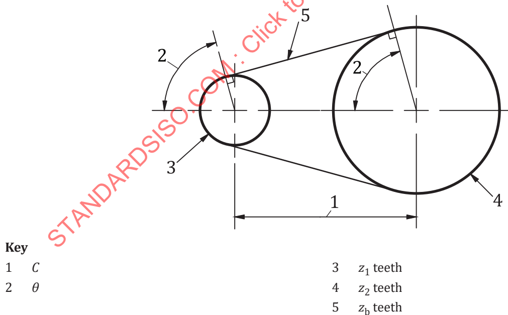
Figure 1 — Centre distance
