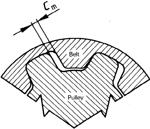
Figure 2 — Clearance between measuring pulley and belt
