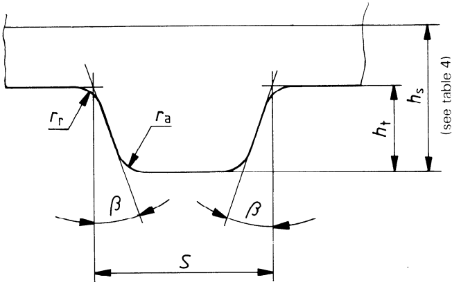
Figure 1 — Tooth profile
