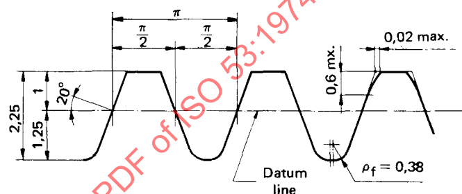
FIGURE 1 Representation of the profile of module m = 1 or of diametral pitch P = 1
