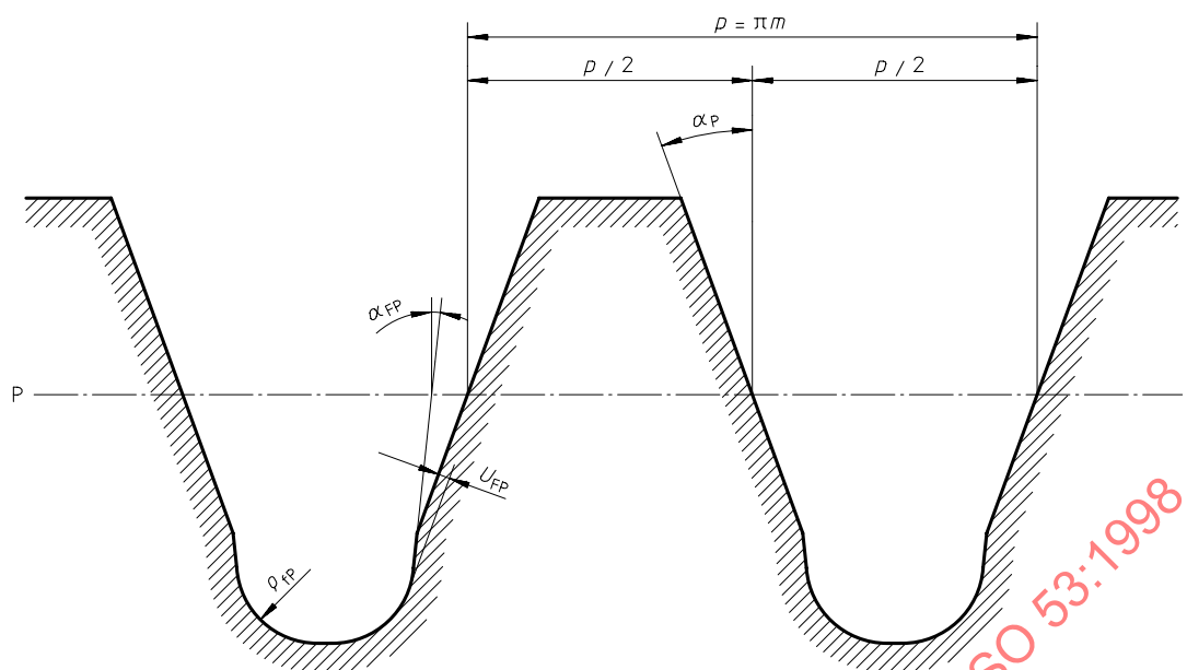
Figure A.1 — Basic rack tooth profile with a chosen undercut
