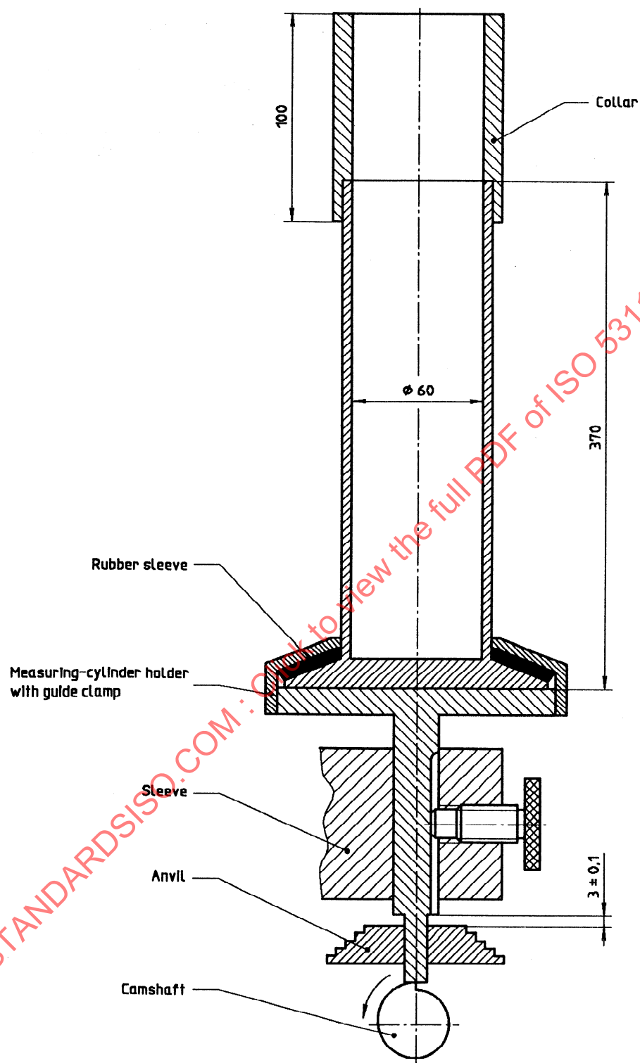
Figure 1 — Apparatus for the determination of bulk density (tapped) by machine tapping
