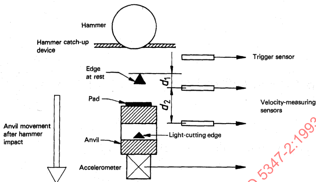
Figure 1 — Shock machine
