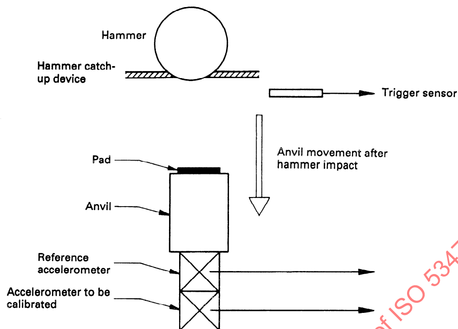
Figure 1 — Shock machine
