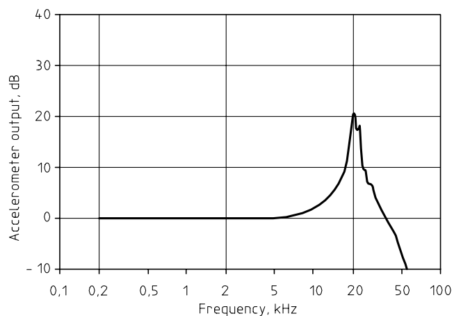
Figure 9 — Typical frequency response of a representative magnetically mounted accelerometer relative to the absolute acceleration of the structure at its attachment
