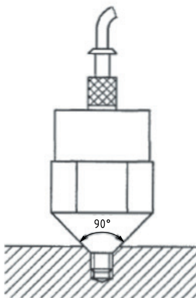
Figure 10 — Mounting by conical bolting
