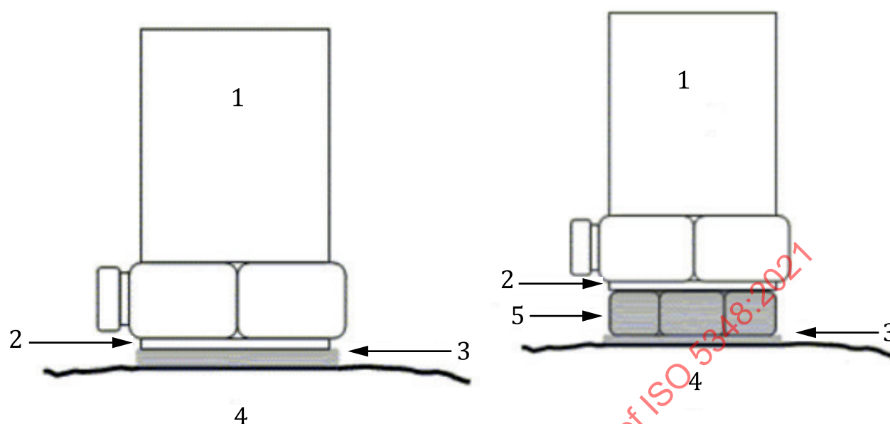
a) Transducer directly glued
