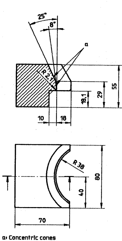
Figure B.3 — Test body for free space at boot toe, type C
