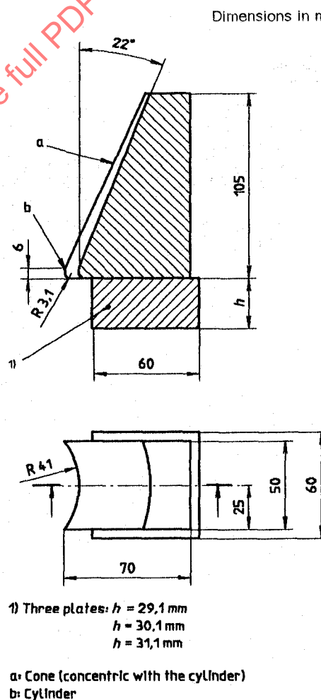
Figure B.2 — Test body for free space at rear of boot, type A
