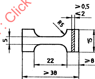
Figure 10 — PTFE specimen
