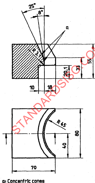
Figure B.1 — Test body for the free space at boot toe, type A
