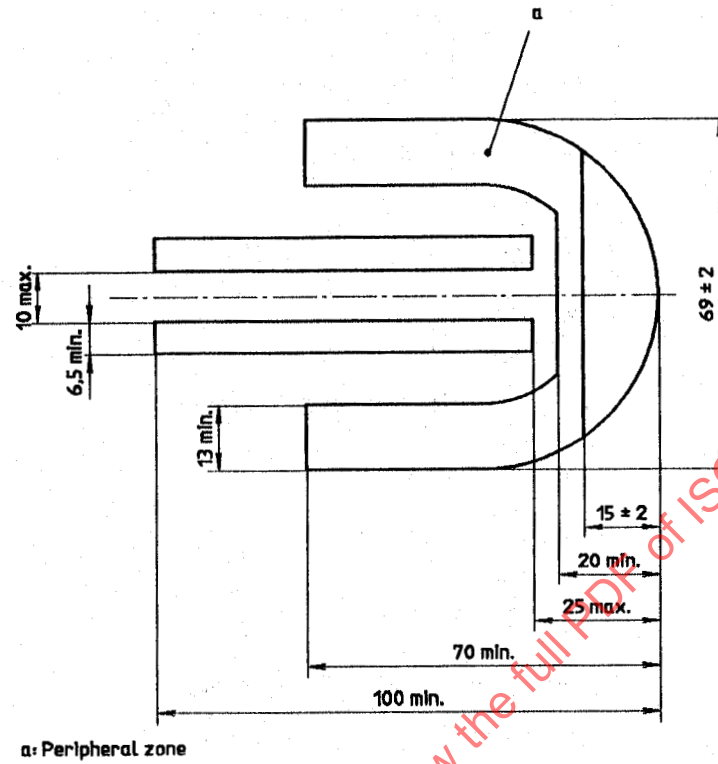
Figure 8 — Example of minimum bearing surface at heel, type A
