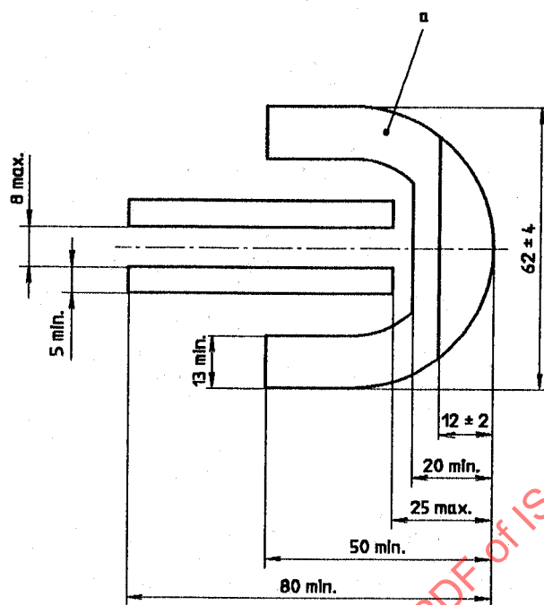
Figure 9 — Example of minimum bearing surface at heel, type C
