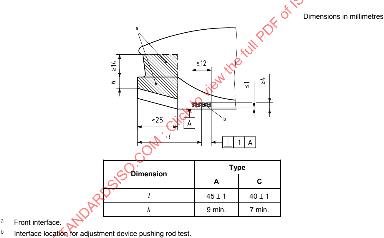
Figure 15 — Front interface and interface location for adjustment device pushing rod test
