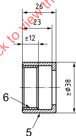
c) Female component — Taper and socket (only essential dimensions shown) a
