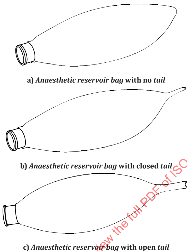
Figure 2 — Examples of anaesthetic reservoir bags with and without tails
