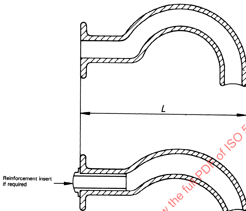
Figure 1 — Length for size designation of airways
