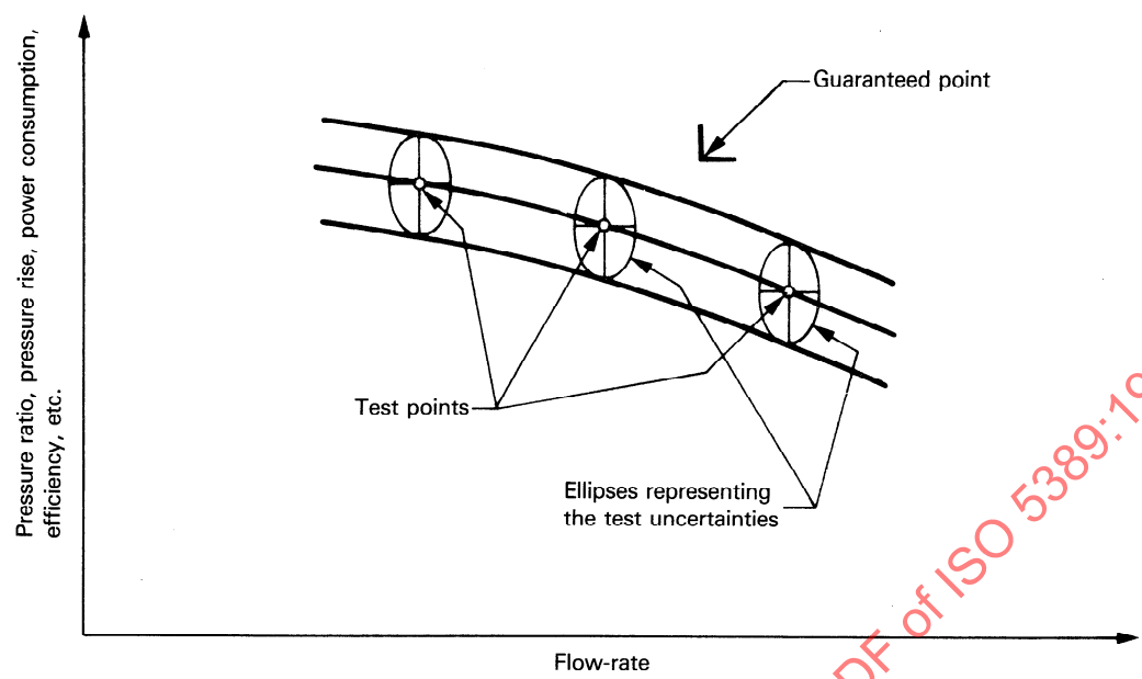
Figure 3 — Comparison of a single guaranteed point with a test curve
