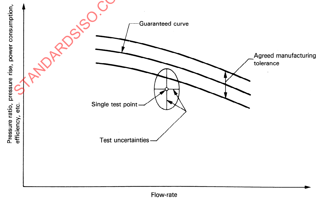
Figure 4 — Comparison of a single test point with a guaranteed curve
