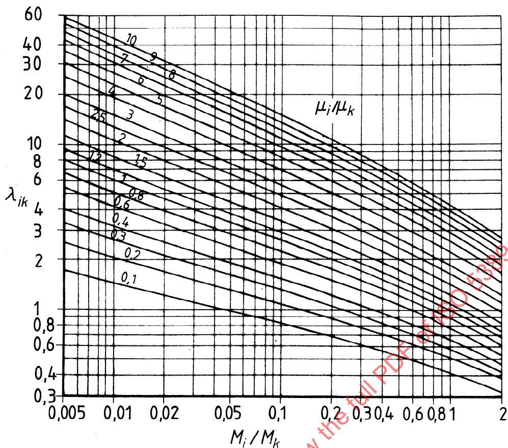
Figure B.1 — Diagram for the determination of the viscosity of gas mixtures
