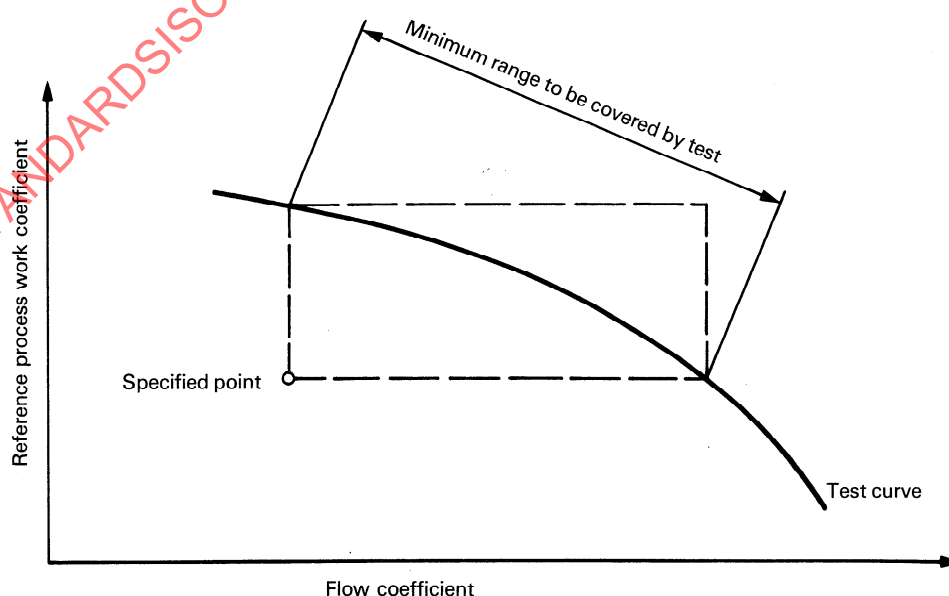
Figure 2 — Minimum range to be covered by the test
