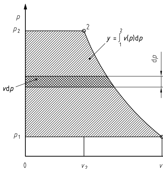
Figure E.7 — Specific compression work, area in the p, v diagram
