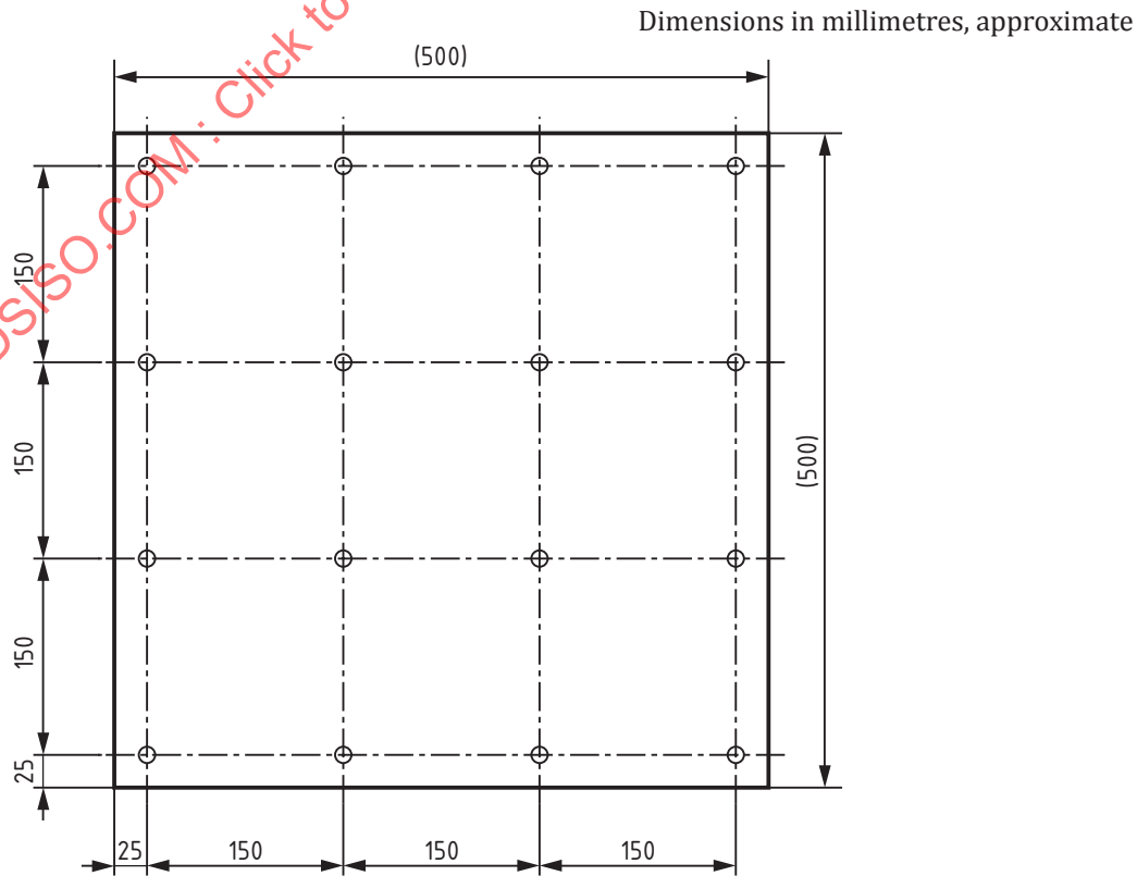
Figure E.3 — Example of base, nail plan
