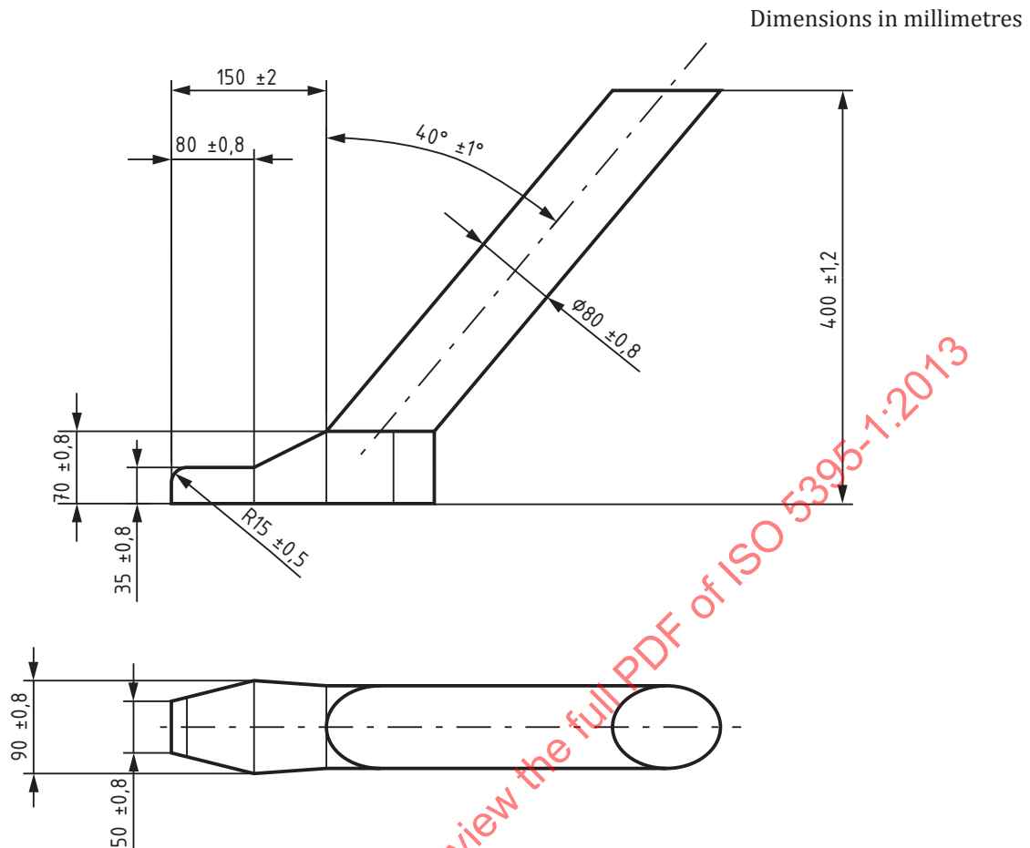
Figure C.1 — Foot probe
