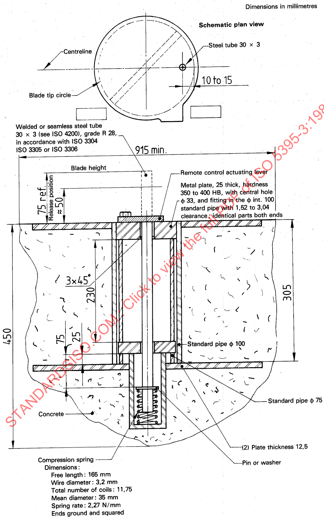
Figure 1 — Impact test fixture
