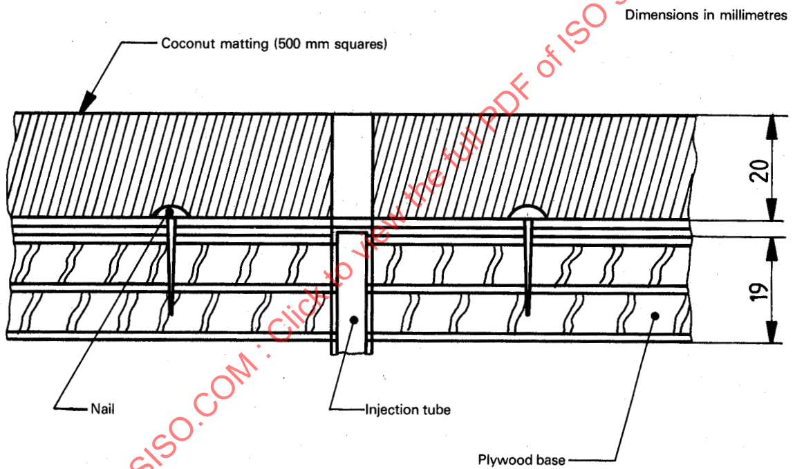
Figure 4 — Thrown object test — Fixture base detail
