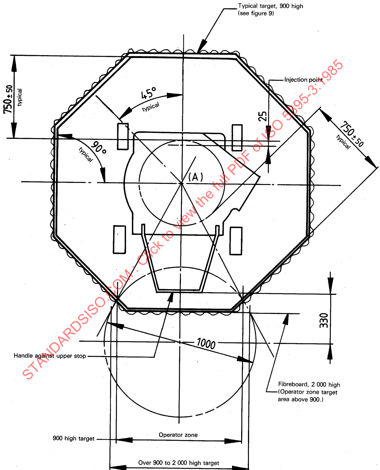
Figure 6 – Thrown object test – Single spindle pedestrian control mower target location
