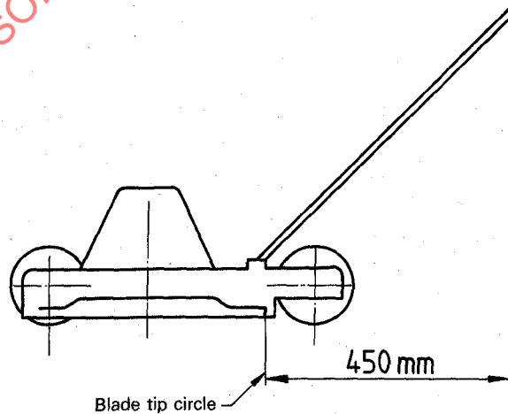
Figure 11 — Handle length
