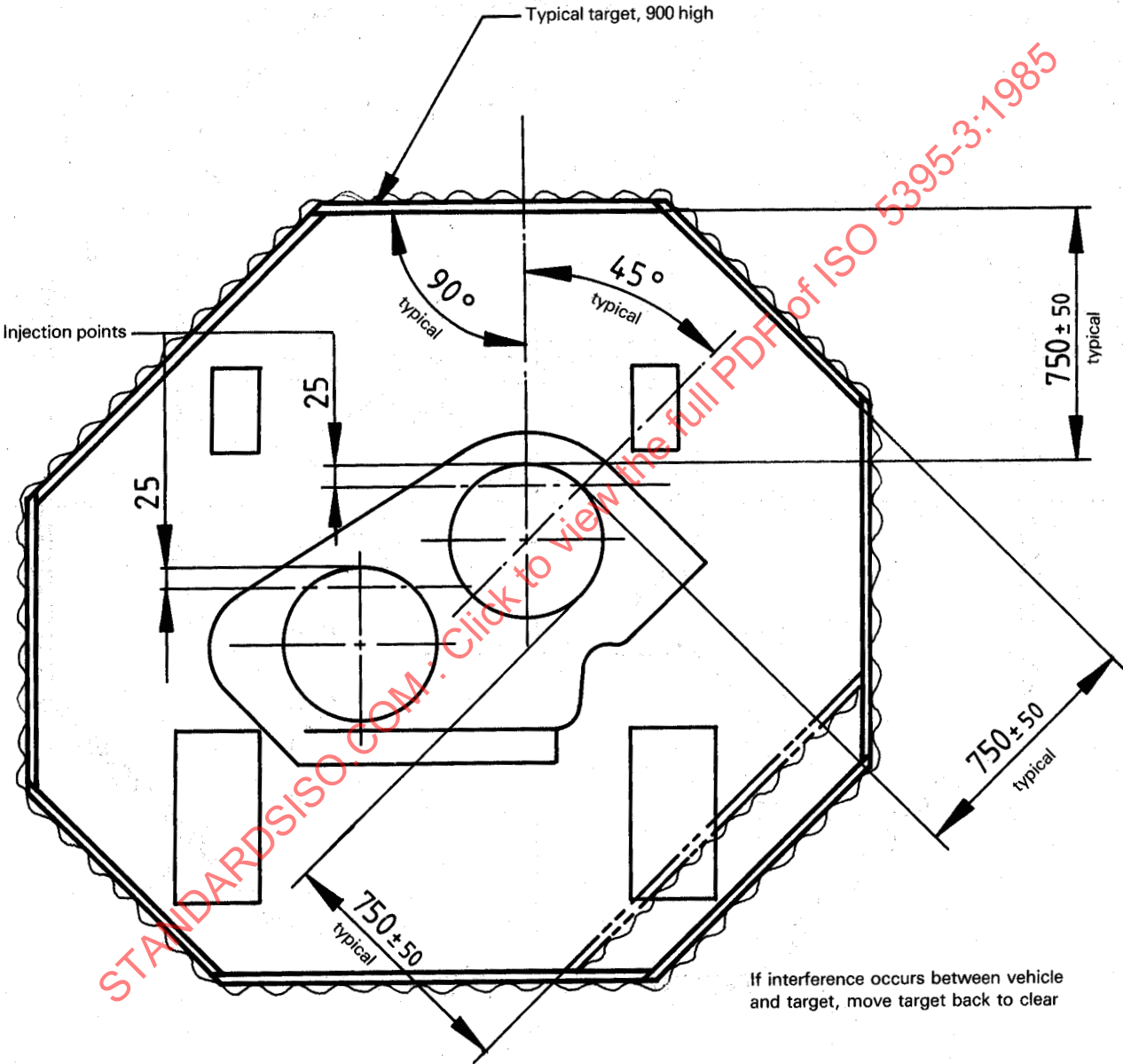
Figure 9 — Thrown object test — Multisindle ride-on mower target location
