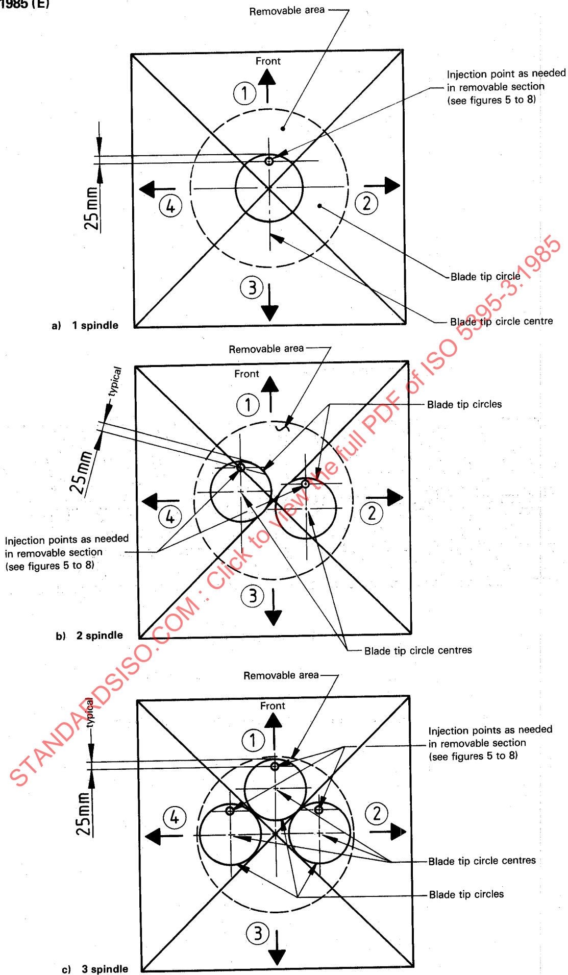
Figure 5 — Thrown object test fixture — Layout of base
