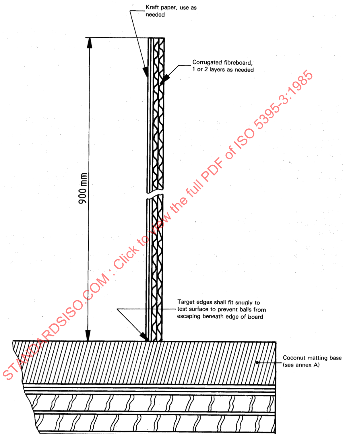
Figure 10 — Thrown object test fixture — Section through test panels (target)
