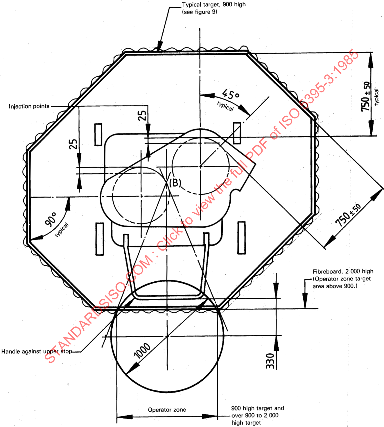
Figure 7 — Thrown object test — Multispindle pedestrian control mower target location
