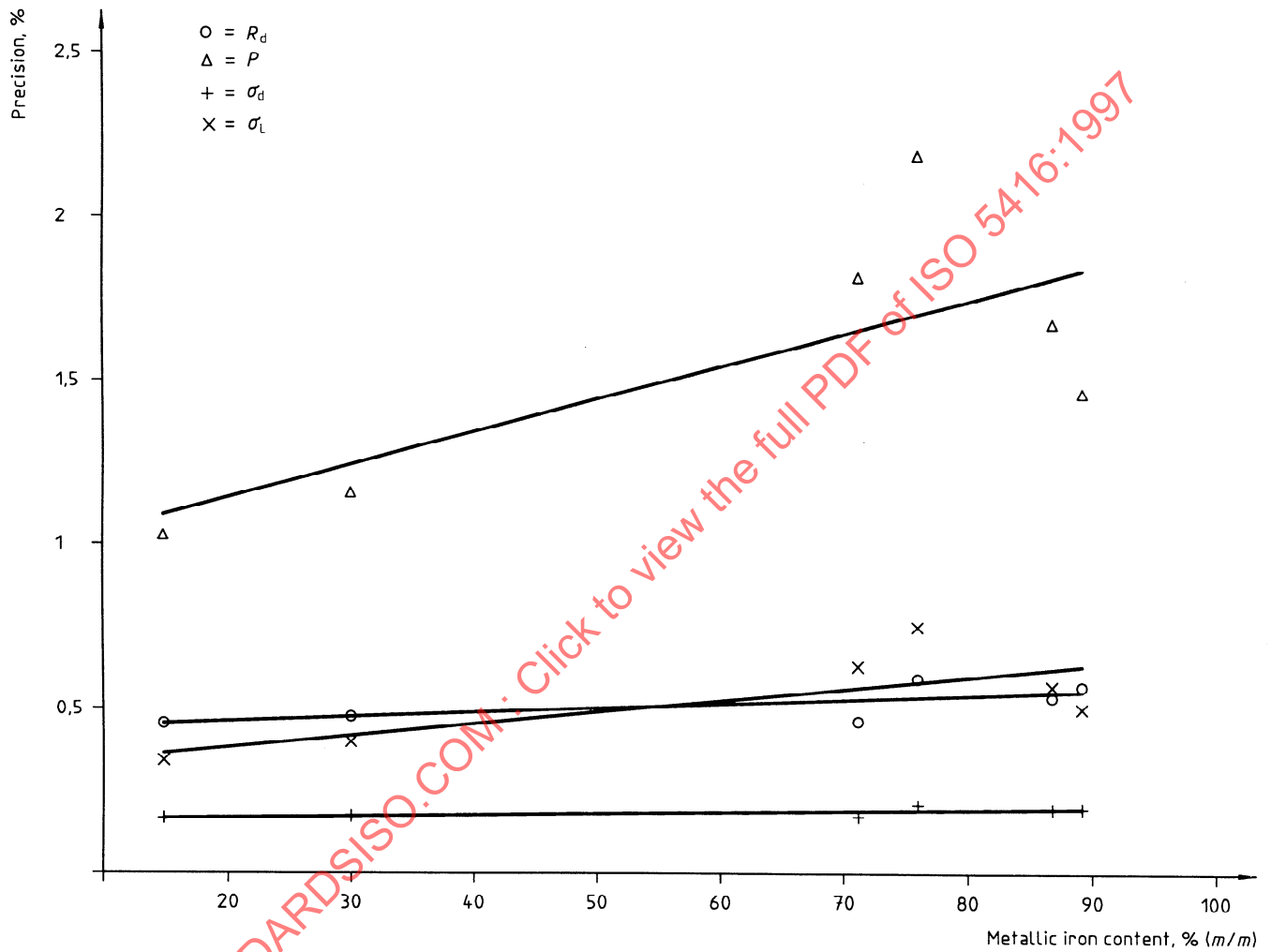
Figure C.1 — Least-squares fit of precision against X for metallic iron
