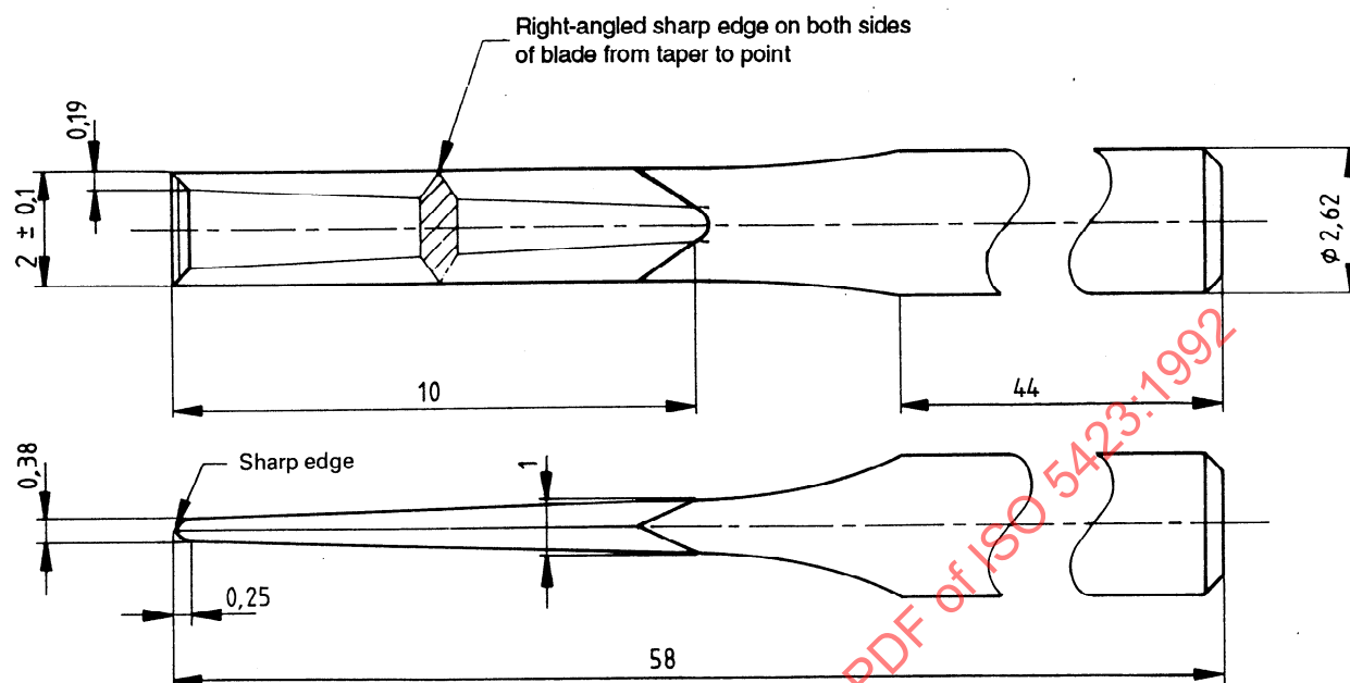
Figure C.2 — Piercing chisel
