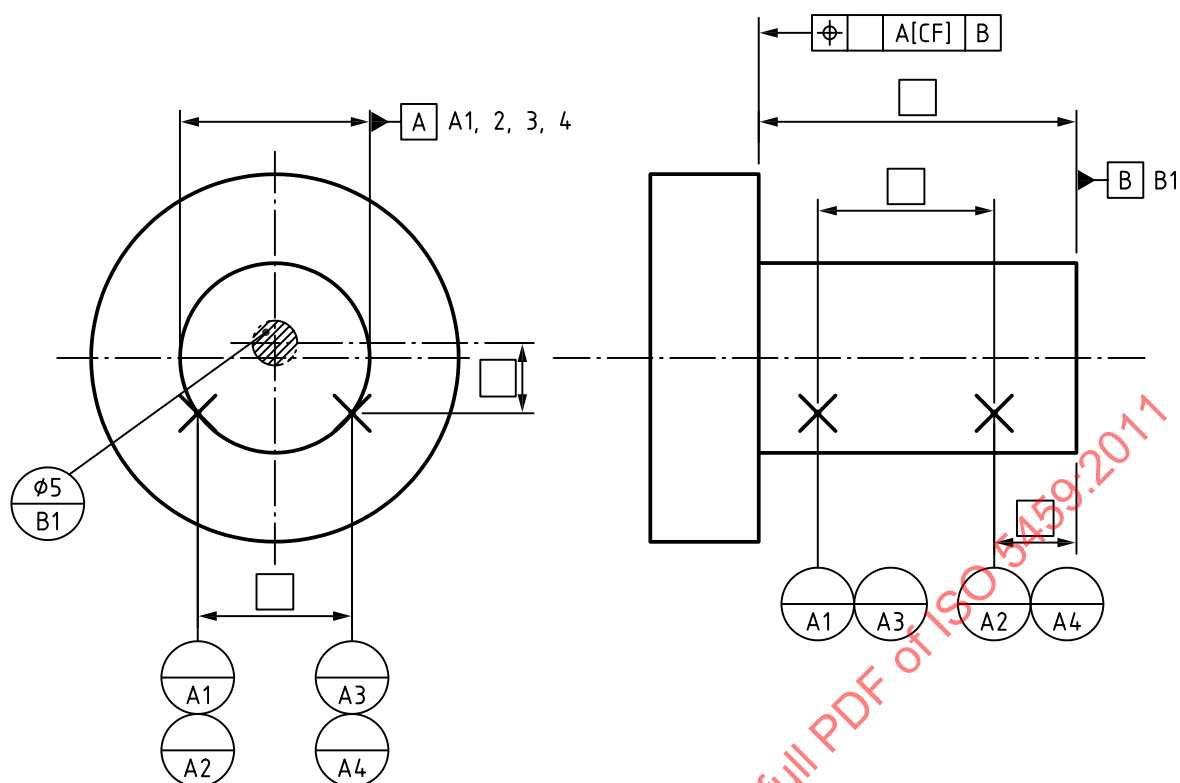
Figure 26 — Example of indication of datum with modifier [CF]
