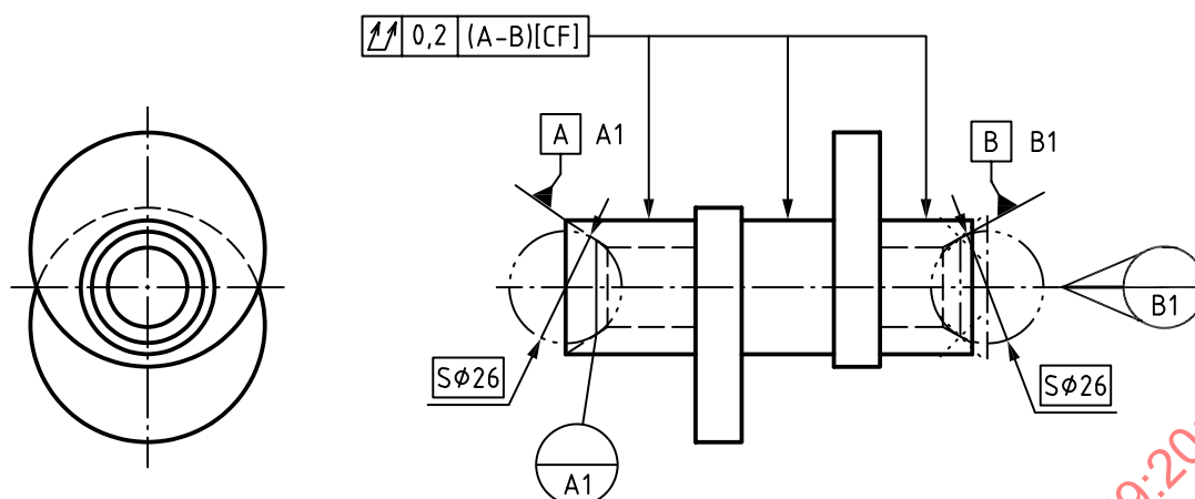
Figure 30 — Example of datum system in which the datum target is indicated
