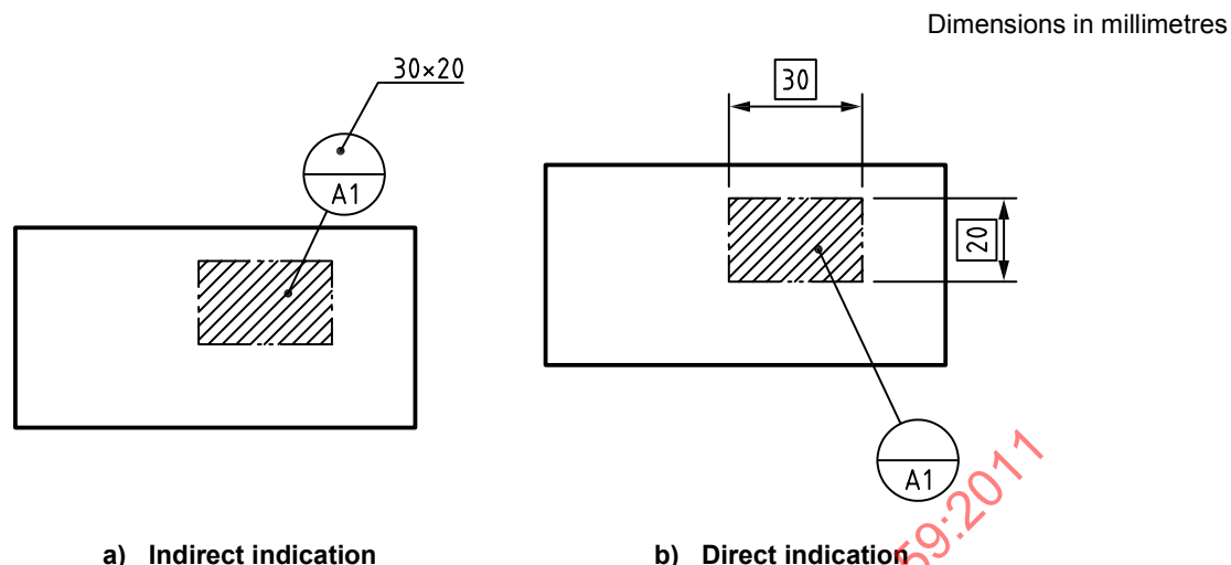
Figure 25 — Indication of dimensions of a rectangular area
