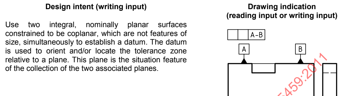
Figure C.23 — Two coplanar planes — Input for reading (drawing indication) and for writing (design intent)
