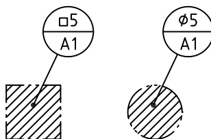
Figure 24 — Indication of dimension of a circular/square area
