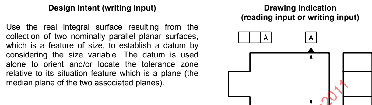
Figure C.19 — Two parallel planes — Input for reading (drawing indication) and for writing (design intent)
