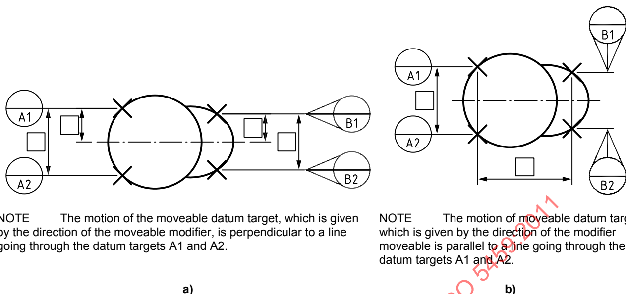
Figure 16 — Example of moveable datum targets
