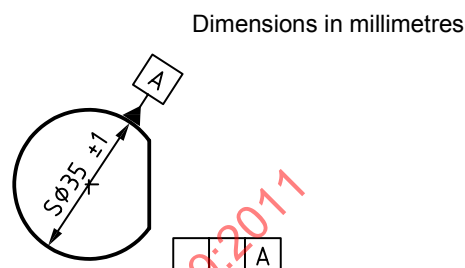
Figure C.7 — Sphere — Input for reading (drawing indication) and for writing (design intent)
