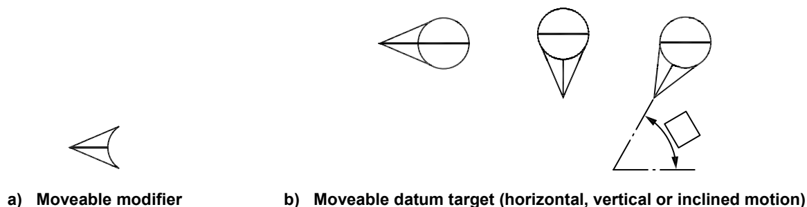
Figure 7 — Moveable modifier and examples of datum target frame with the moveable modifier
