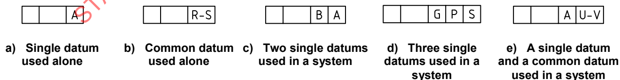
Figure 31 — Examples of indication of datums in the tolerance frame
