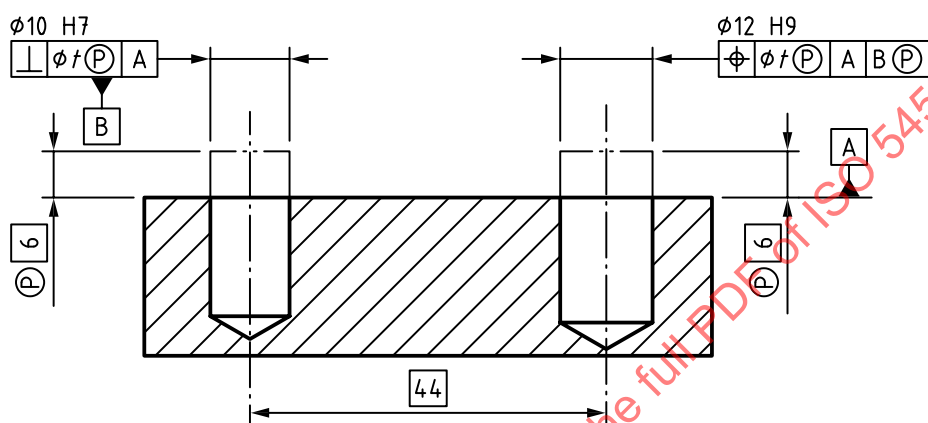
Figure 39 — Example of application of modifier \textcircled{P} on the secondary datum
