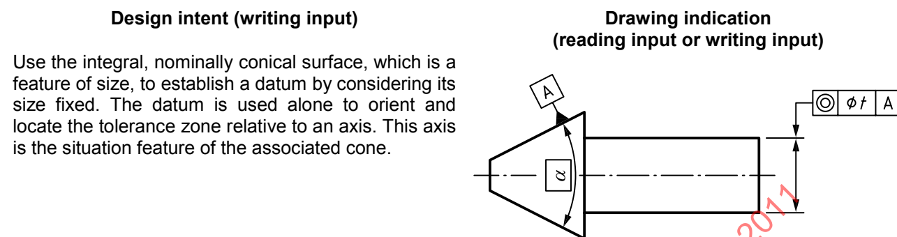
Figure C.11 — Obvious situation feature — Input for reading (drawing indication) and for writing (design intent)
