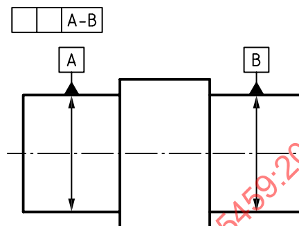
Figure C.25 — Two coaxial cylinders — Input for reading (drawing indication) and for writing (design intent)
