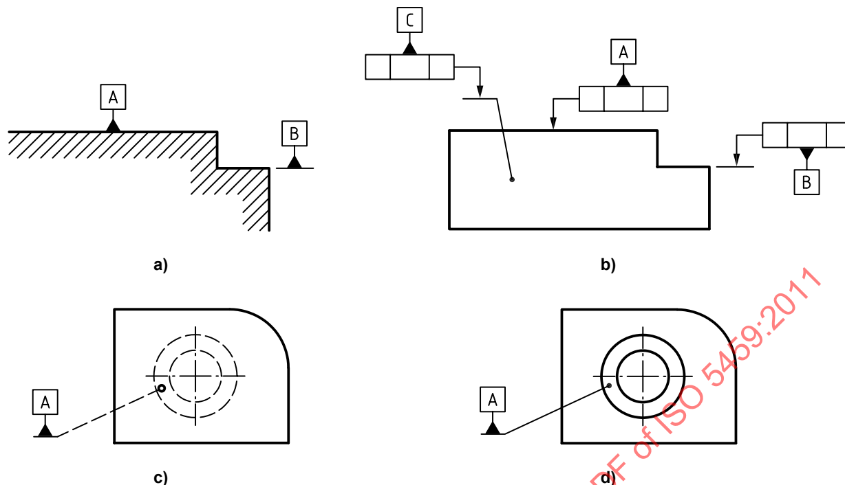
Figure 19 — Attachment of a datum indicator for a single feature not considered a feature of size
