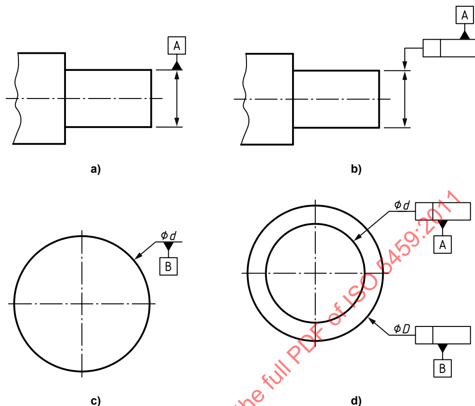
Figure 18 — Attachment of a datum indicator for a single feature considered a feature of size
