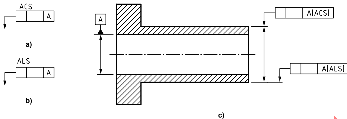
Figure 22 — Indication of [ACS] and [ALS] modifier
