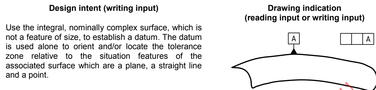
Figure C.15 — Complex surface — Input for reading (drawing indication) and for writing (design intent)
