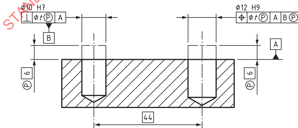
Figure 40 — Example of application of modifier \textcircled{P} on the secondary datum
