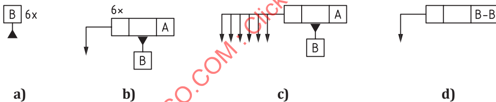
Figure 33 — Examples of complementary indication
