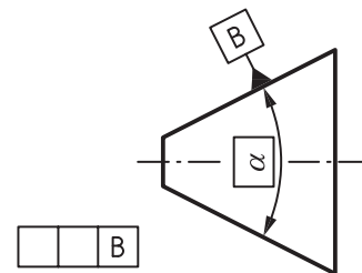
Figure C.5 — Cone — Input for reading (drawing indication) and for writing (design intent)
