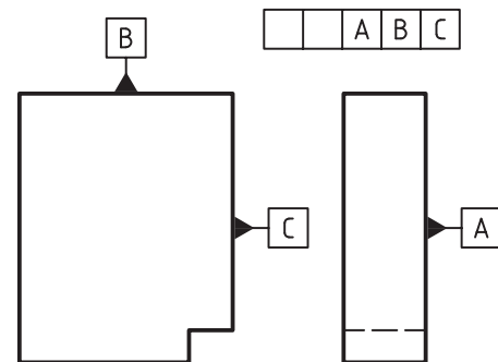
Figure C.35 — Three perpendicular planes — Input for reading (drawing indication) and for writing (design intent)
