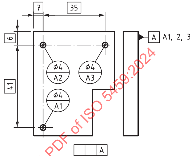
Figure C.21 — Three datum targets on a plane — Input for reading (drawing indication) and for writing (design intent)
