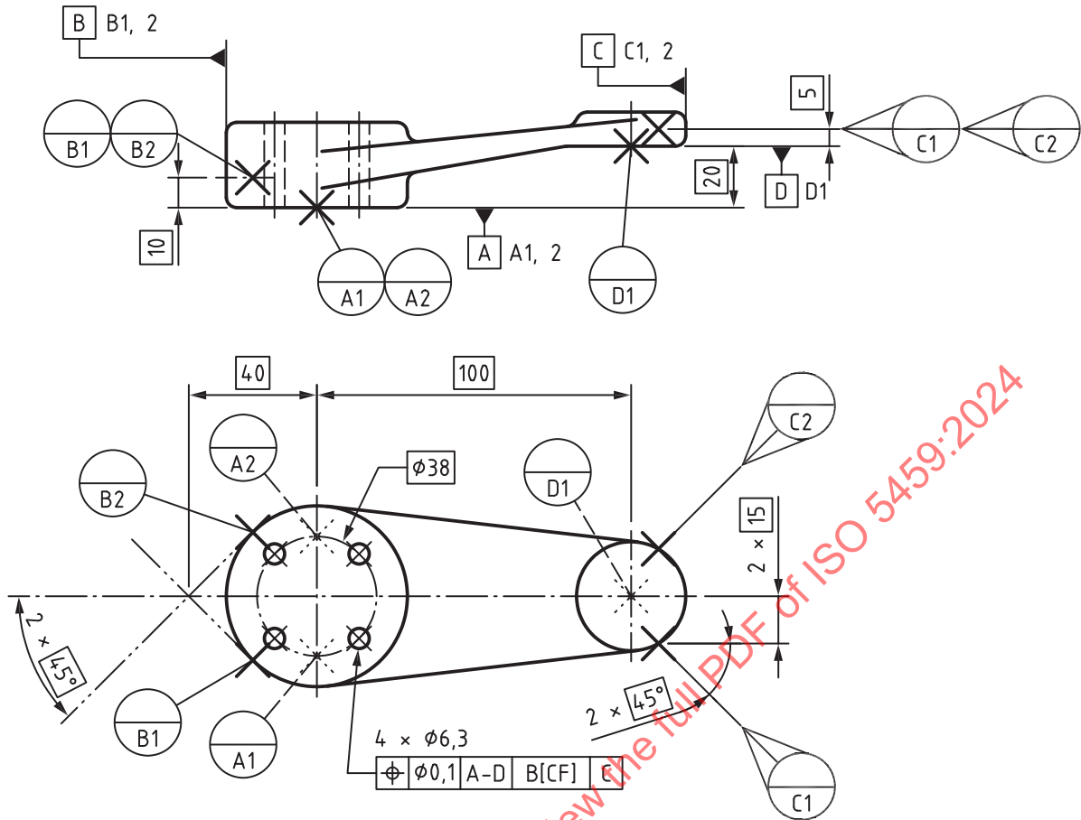
Figure 28 — Example of datum system established from datum targets
