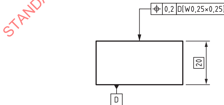
Figure 45 — Example of a special specification operator for datum with filtration specification elements
