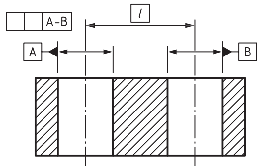
Figure C.29 — Two parallel cylinders — Input for reading (drawing indication) and for writing (design intent)
