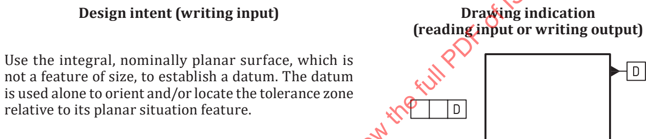
Figure C.1 — Plane — Input for reading (drawing indication) and for writing (design intent)
