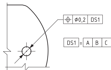
b) Indirect indication of a datum section by using a datum system identifier
