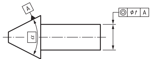
Figure C.11 — Obvious situation feature — Input for reading (drawing indication) and for writing (design intent)
