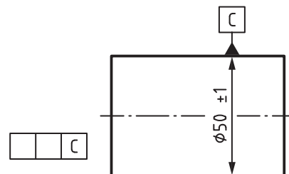
Figure C.3 — Cylinder — Input for reading (drawing indication) and for writing (design intent)
