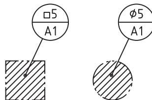
Figure 25 — Indication of dimension of a circular/square area
