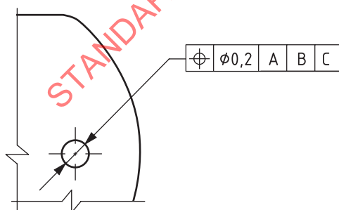
a) Direct indication of a datum section
