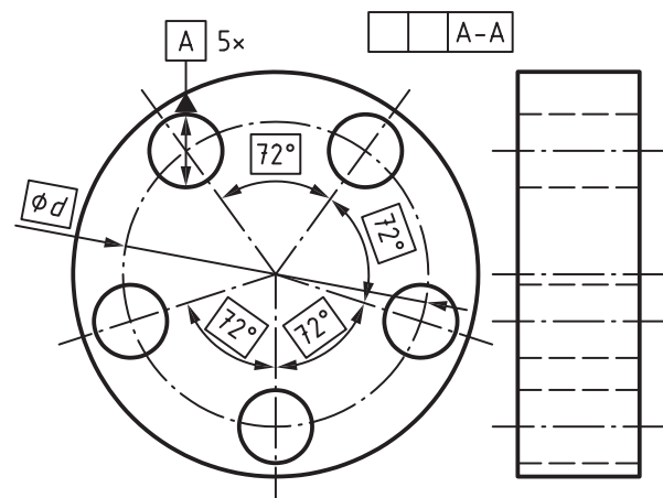
Figure C.31 — Pattern of five cylinders — Input for reading (drawing indication) and for writing (design intent)
