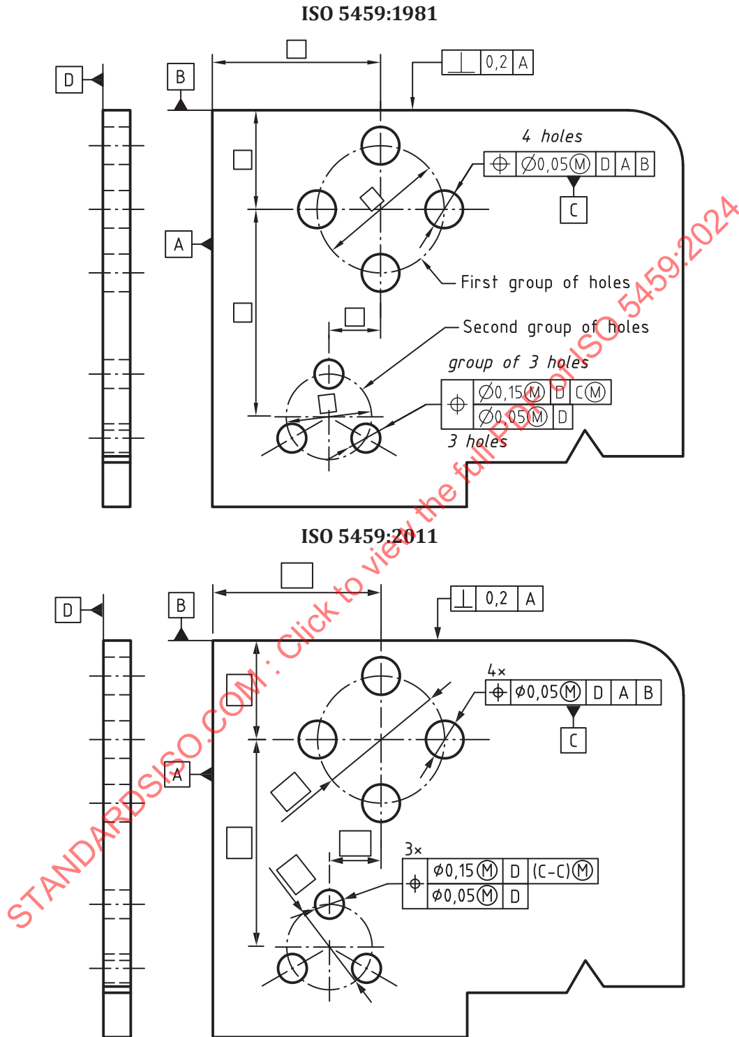
Figure D.3 — Indication of a common datum
