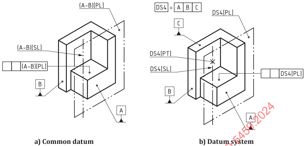
Figure 44 — Example of indication of the situation features constituting a common datum or a datum system
