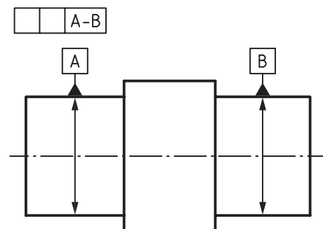
Figure C.25 — Two coaxial cylinders — Input for reading (drawing indication) and for writing (design intent)
