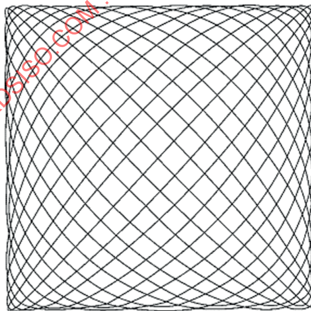
Figure 1 — Lissajous figure
