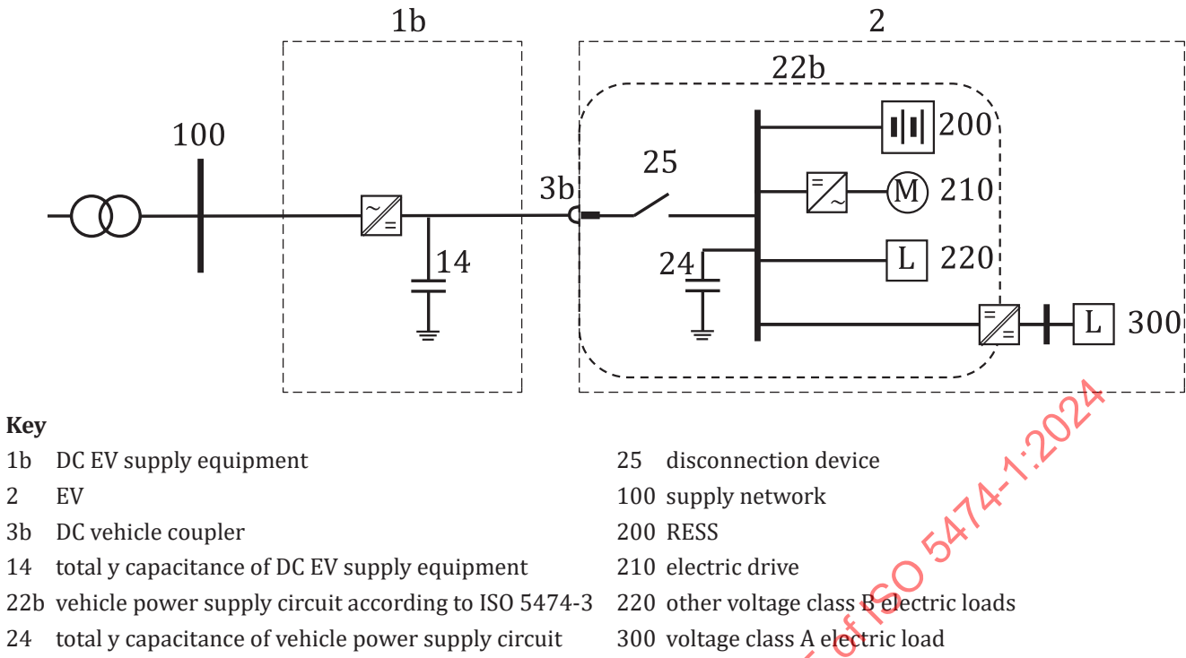
Figure 3 — Single-line diagram of example of DC power transfer system
