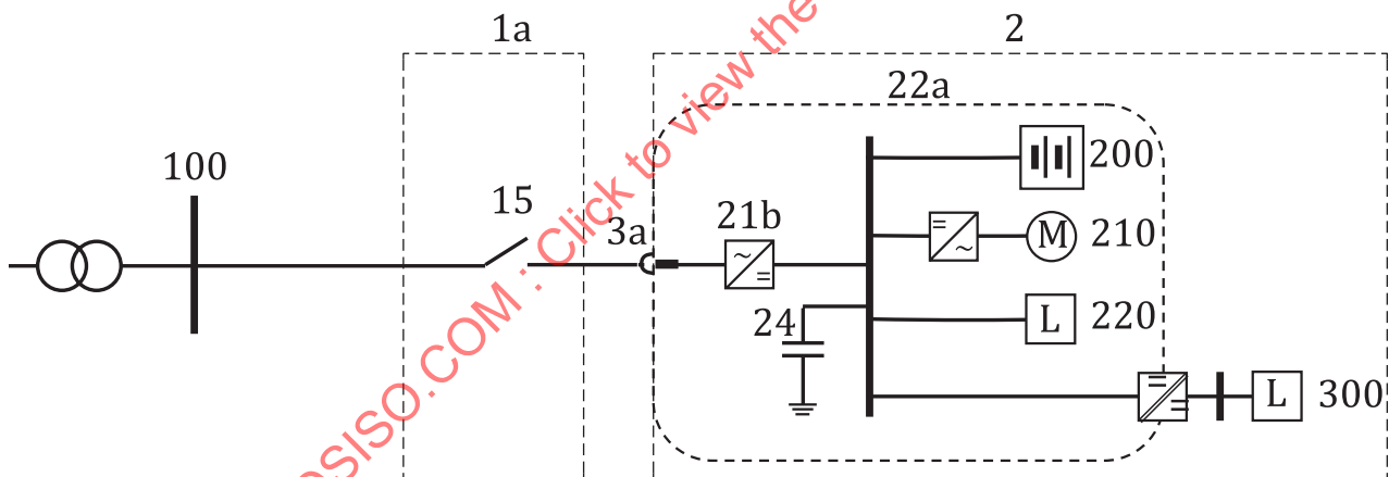
Figure 1 — Single-line diagram of example of AC power transfer system using charger with at least simple separation
