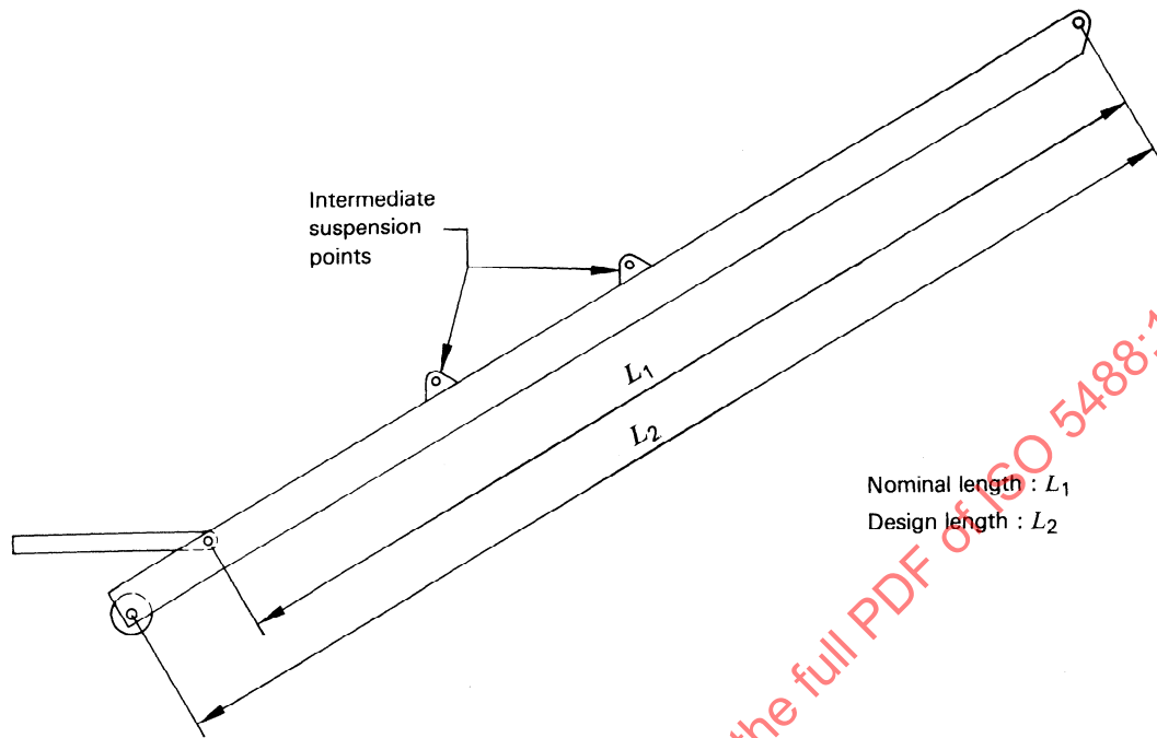
Figure 1 — Single-flight ladder
