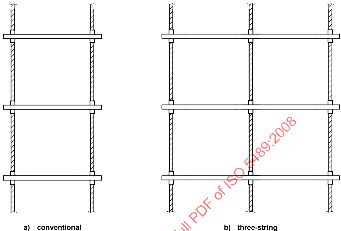
Figure 1 — Embarkation ladders
