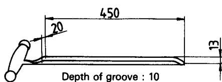
Figure 1 — Sampling spear (open trier)
