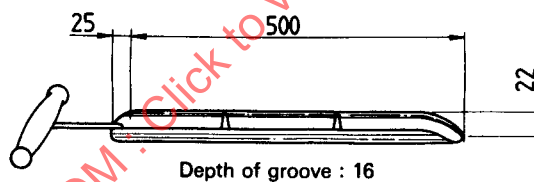
Figure 3 — Divided sampling spear (open trier)
