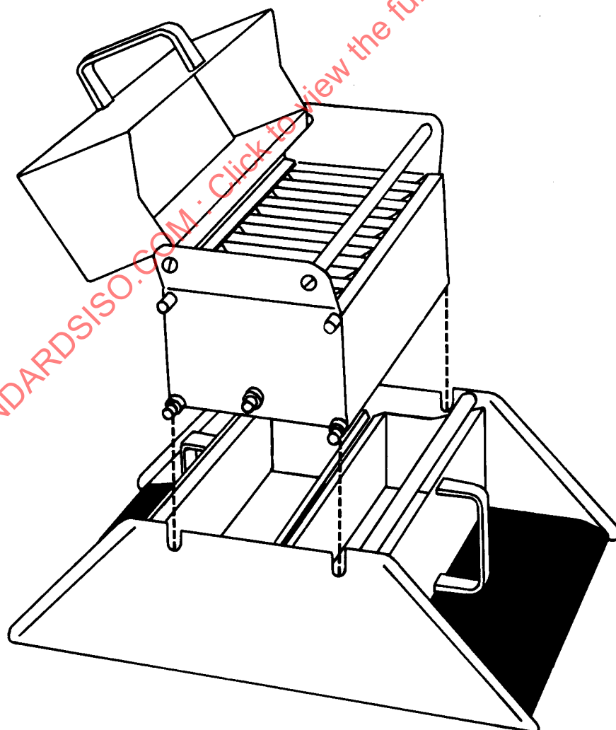
Figure 2 — Multiple slot divider with sorting system
