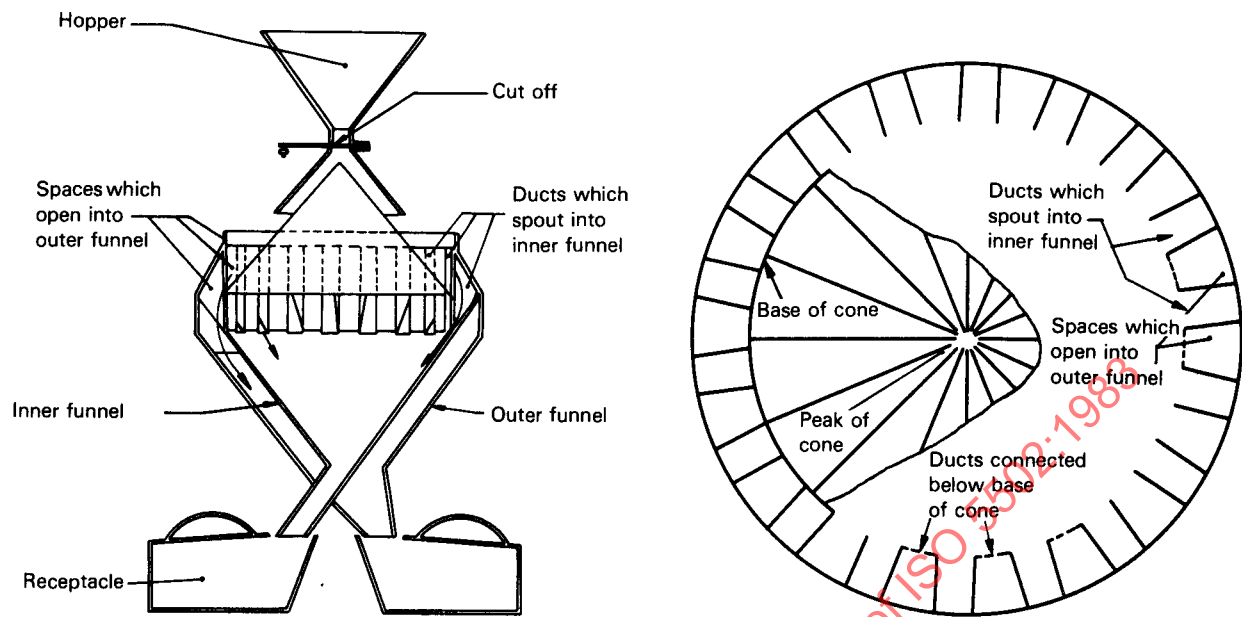
Figure 1 — Conical divider
