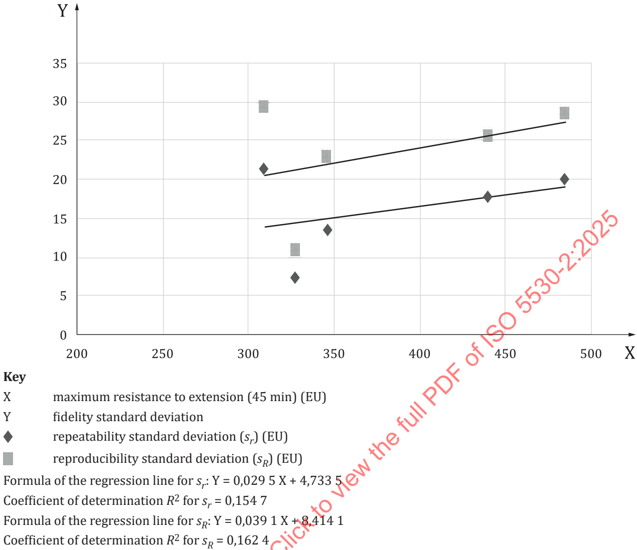
Figure B.10 — Evolution of the fidelity standard deviations as a function of the measured maximum resistance to extension (45 min)
