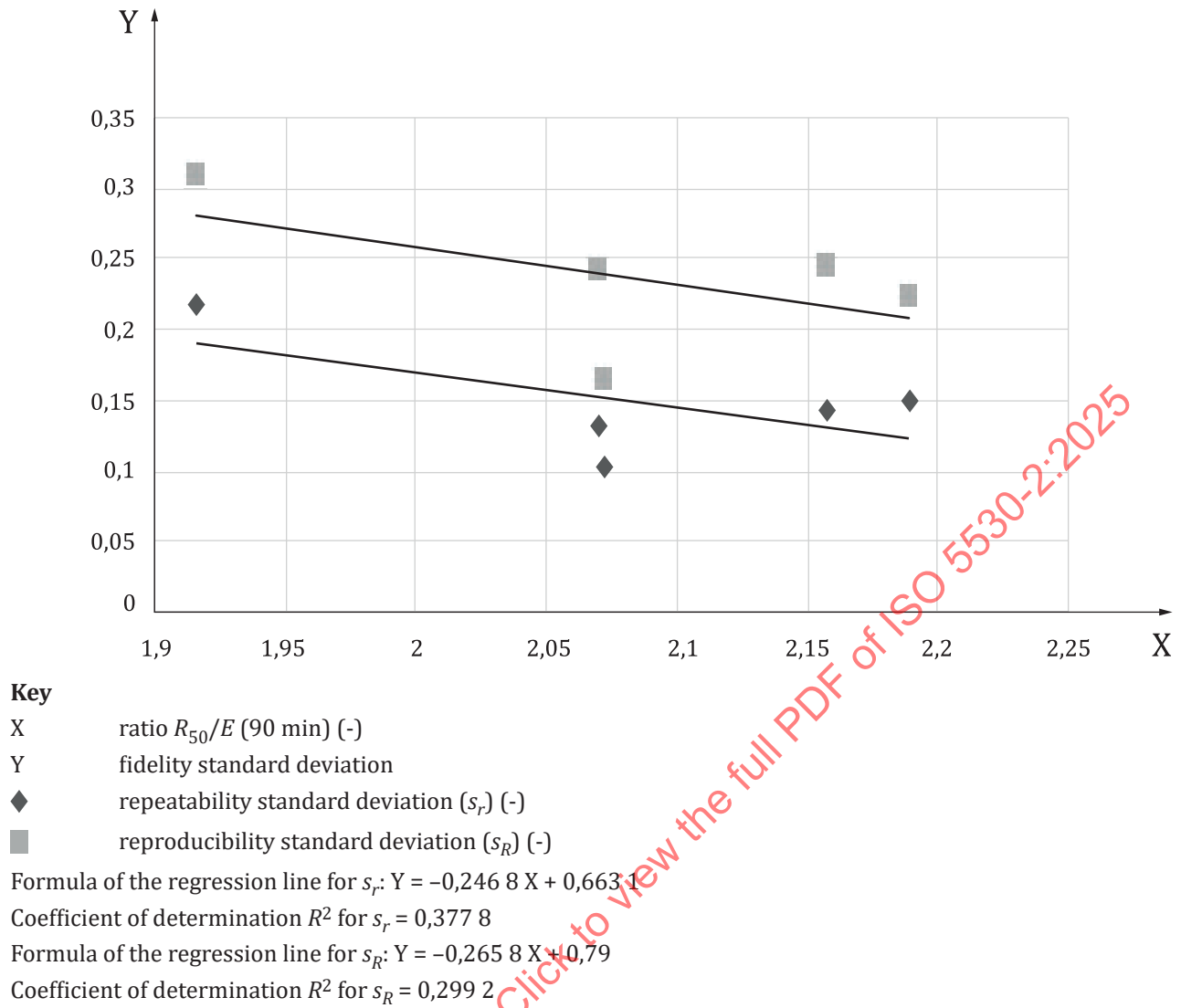
Figure B.14 — Evolution of the fidelity standard deviations as a function of ratio R_{50}/E (90 min)
