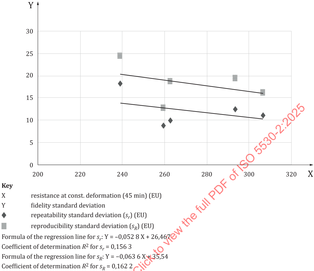
Figure B.7 — Evolution of the fidelity standard deviations as a function of the measured resistance at constant deformation (45 min)
