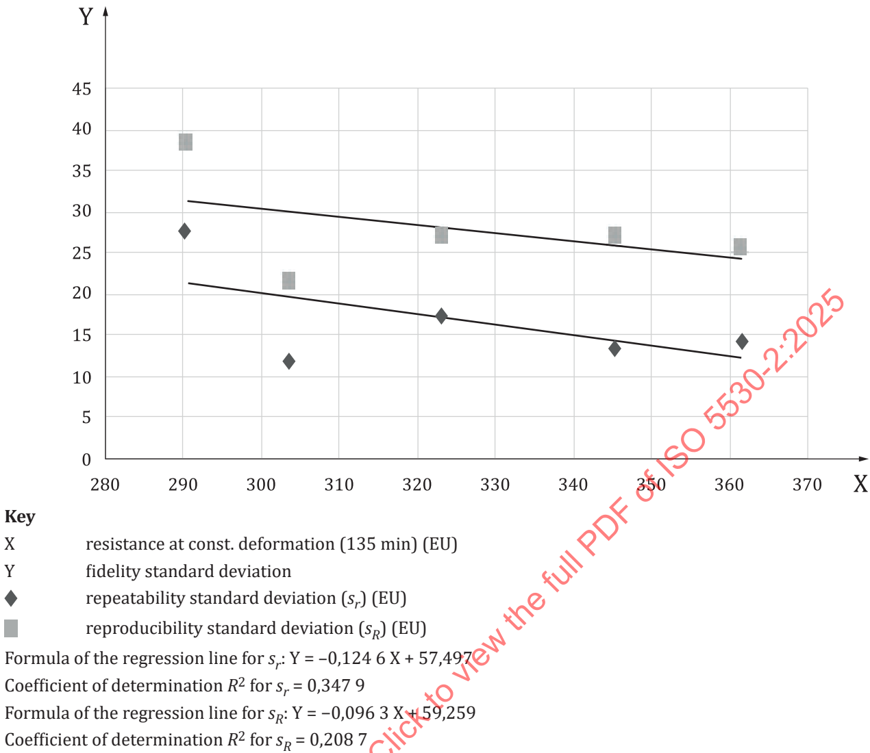
Figure B.9 — Evolution of the fidelity standard deviations as a function of the measured resistance at constant deformation (135 min)
