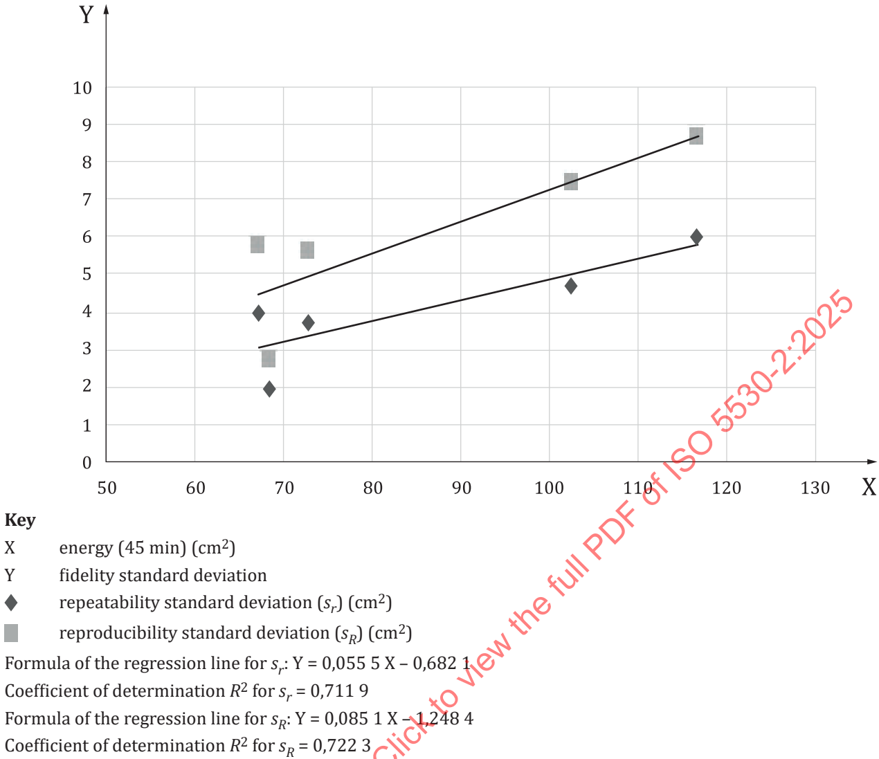
Figure B.1 — Evolution of the fidelity standard deviations as a function of the measured energy (45 min)
