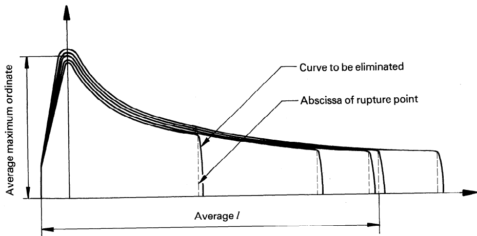
Figure 3 — Curves obtained by using a water pressure gauge
