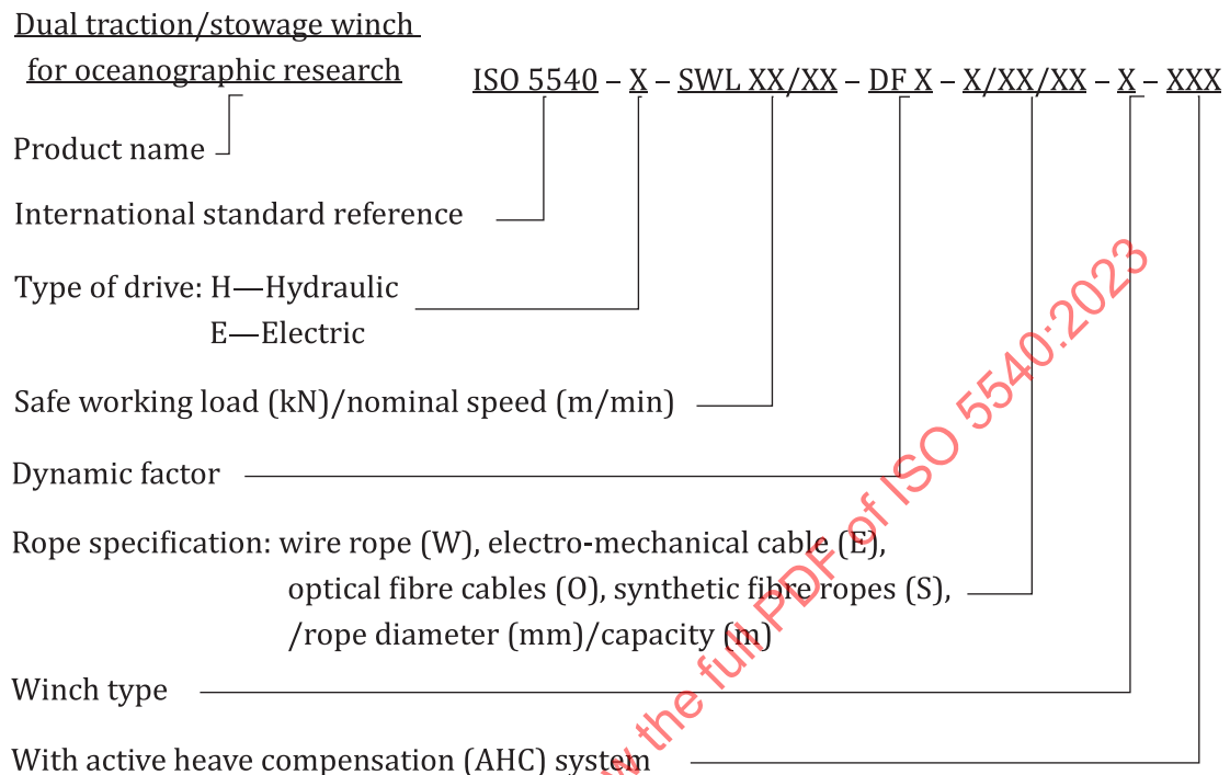
Figure 2 — Model designation of dual traction/traction winches
