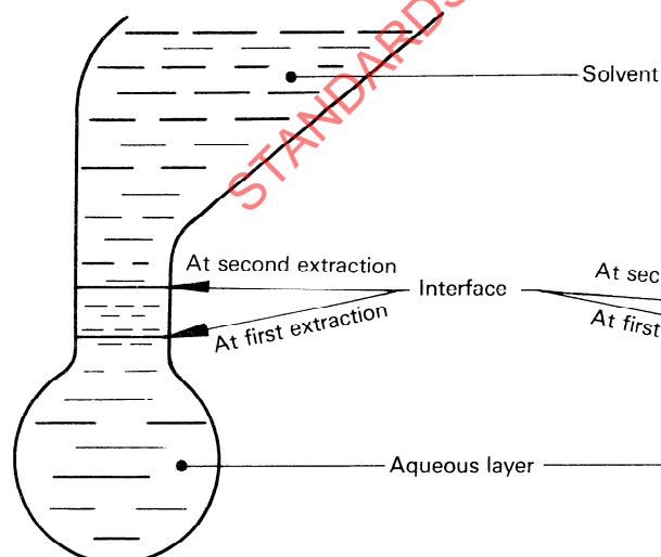
Figure 1 — Before decantation (8.5.8, 8.5.11)
