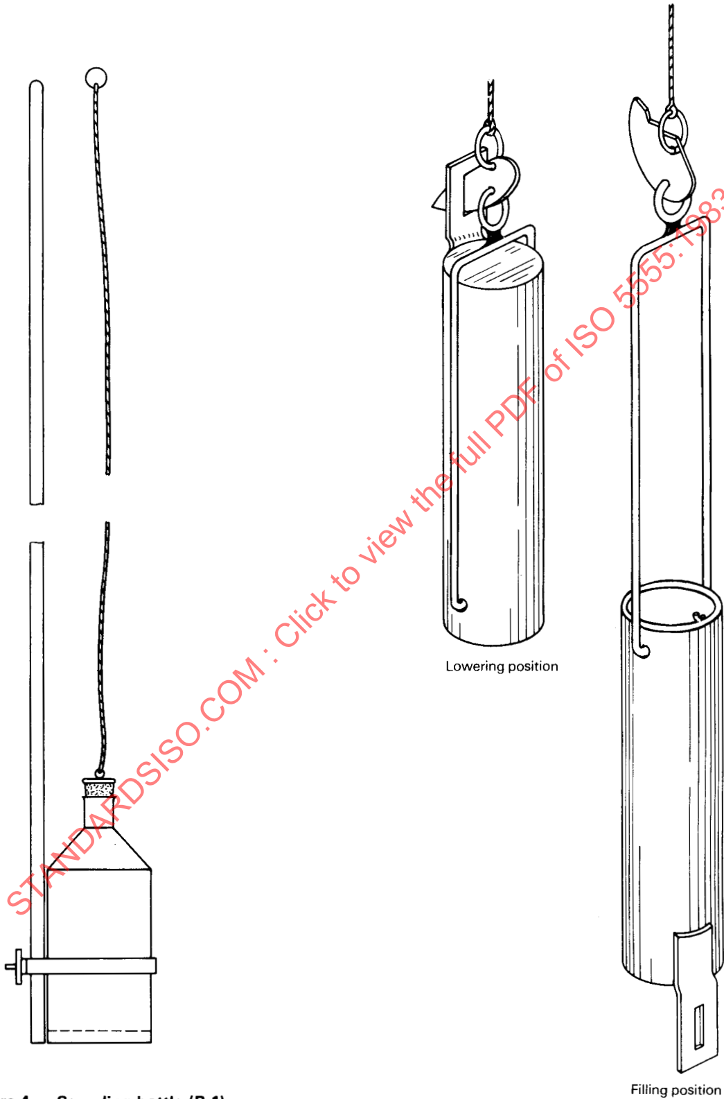
Figure 4 — Sampling bottle (B.1)
