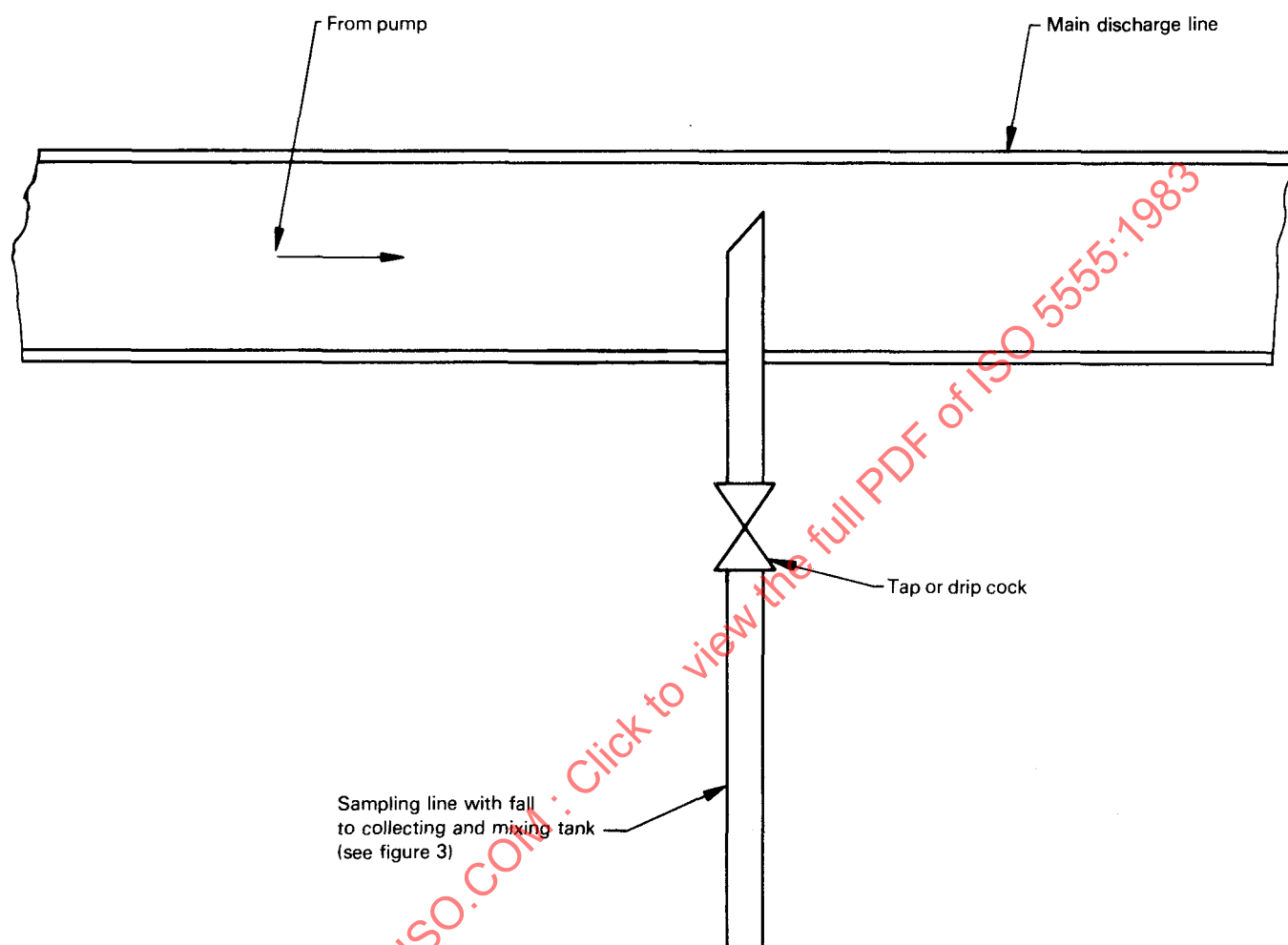
Figure 2 — Sampling line for flow sampling
