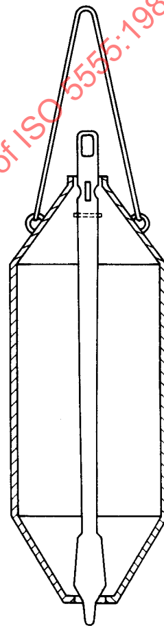
Figure 7 — Bottom sampler or zone sampler (valve type) (B.4) (cross-section)
