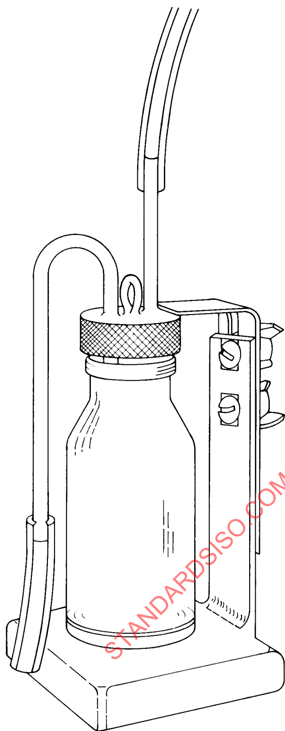
Figure 8 — Bottom sampler or zone sampler (air-tube type) (B.4)
