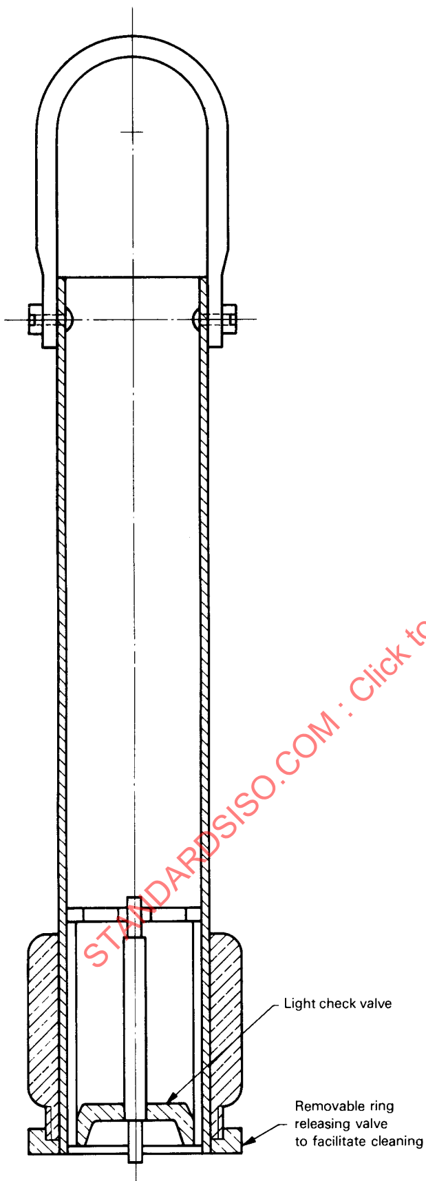
Figure 6 — Valve sampling cylinder (sinker sampler) (B.3)
