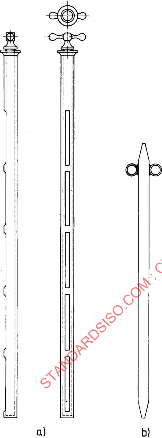
Figure 11 — Sampling tubes (B.6)
