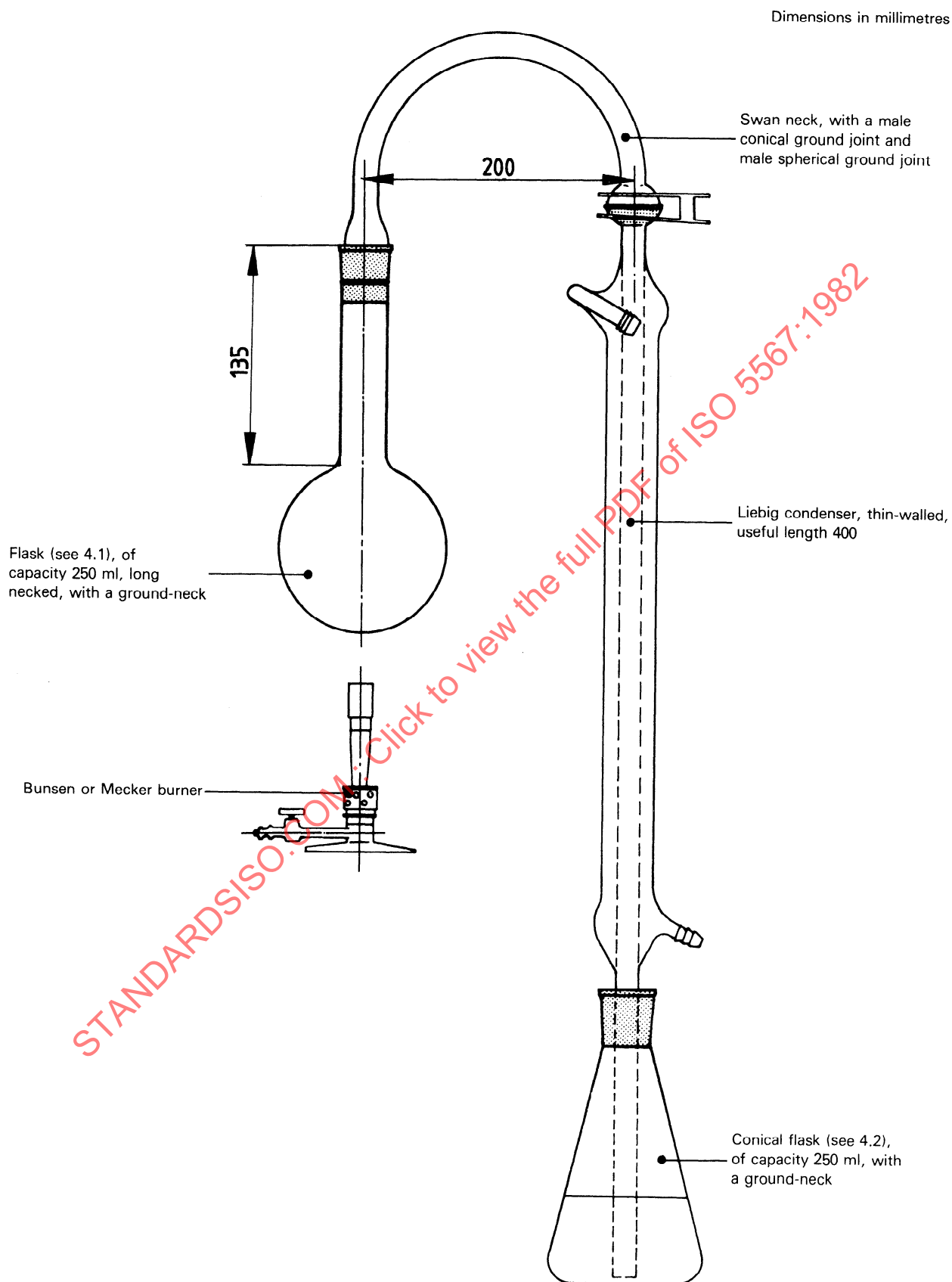
Figure — Allyl sulphide distillation apparatus (recommended)
