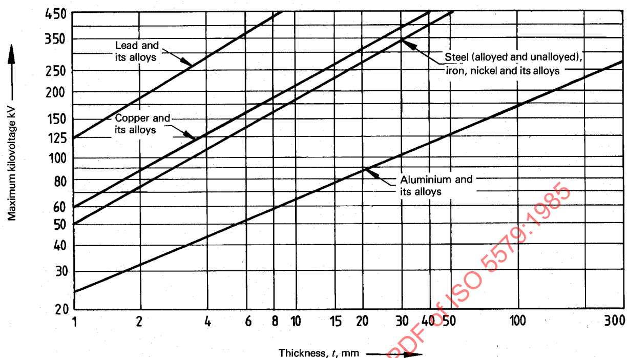
Figure 9 — Maximum kilovoltage for X-rays up to 450 kV for different materials for classes A and B in terms of material thickness t^{(1)}
