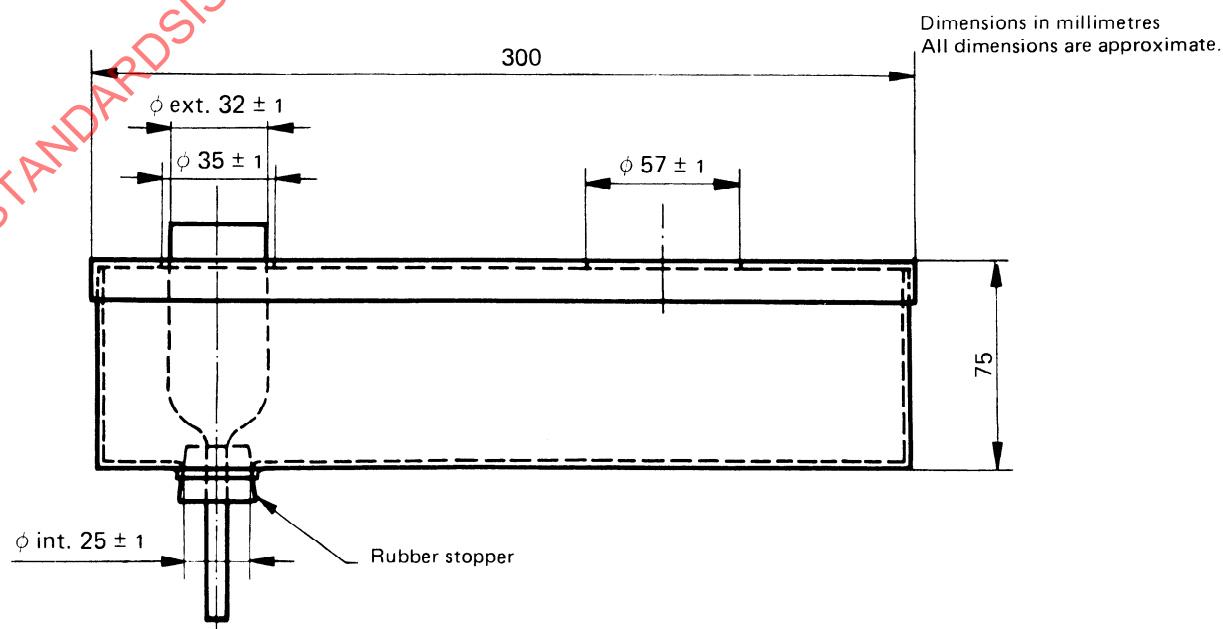
FIGURE 2 – Hot water bath for determination of matter insoluble in hot alcohol (method I)
