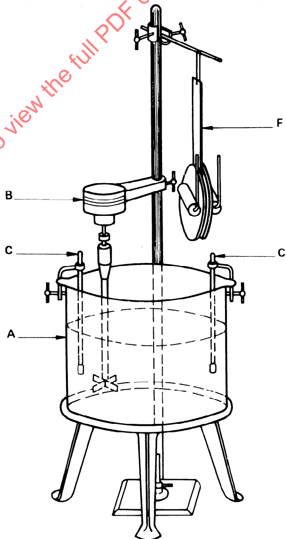
FIGURE 7 — Apparatus for flow test (the test tubes are held in an inclined position on the testing fixture F, for immersion in the oil bath)
