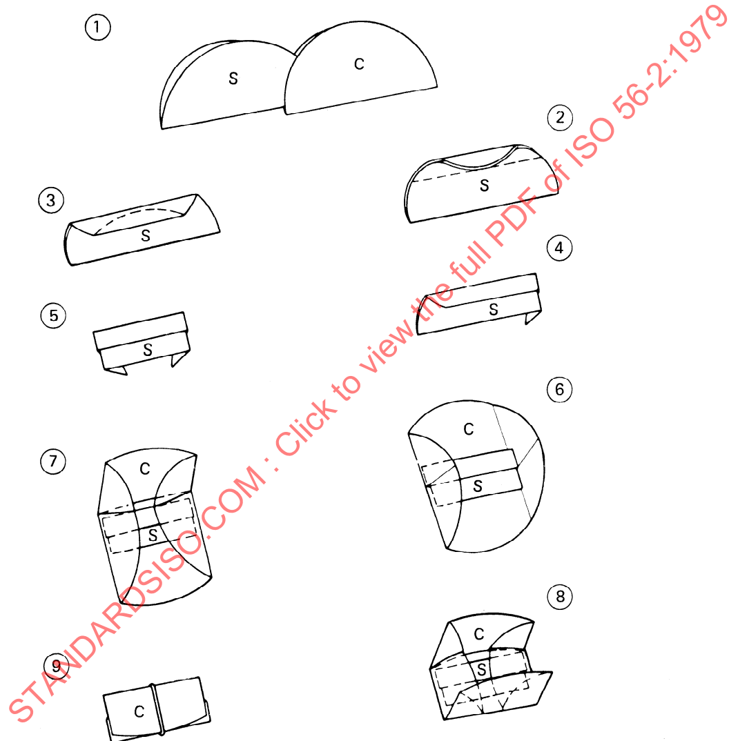
FIGURE 4 — Folding of filter paper
